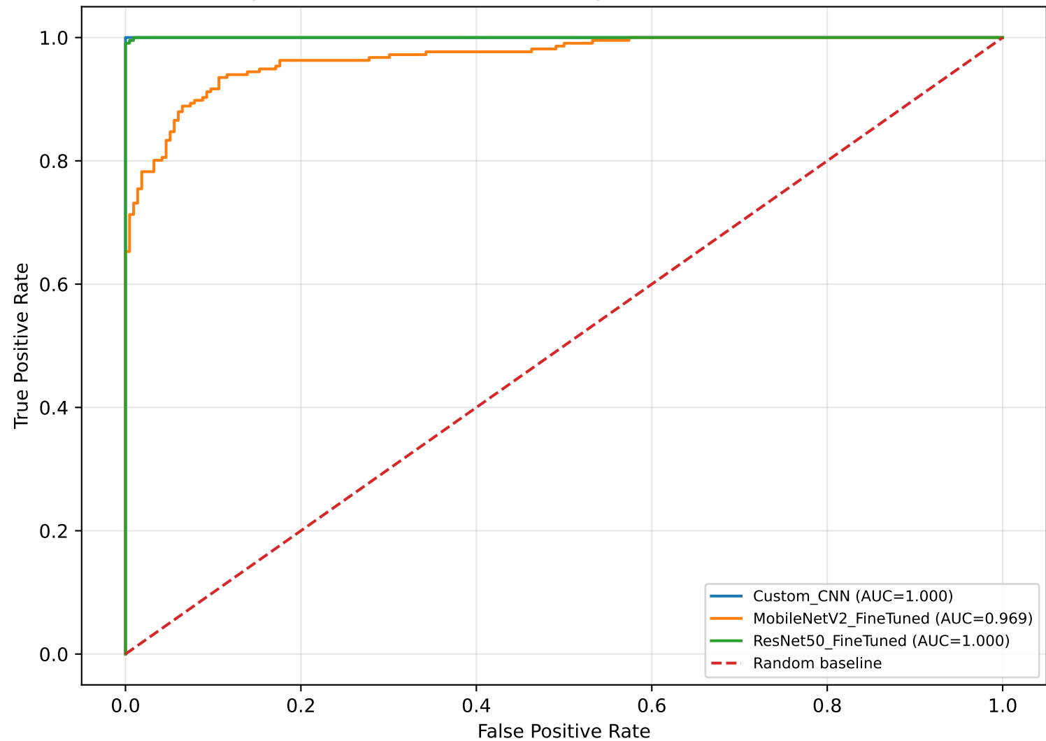
Figure 9. ROC Curves for Final Signature Verification Models
