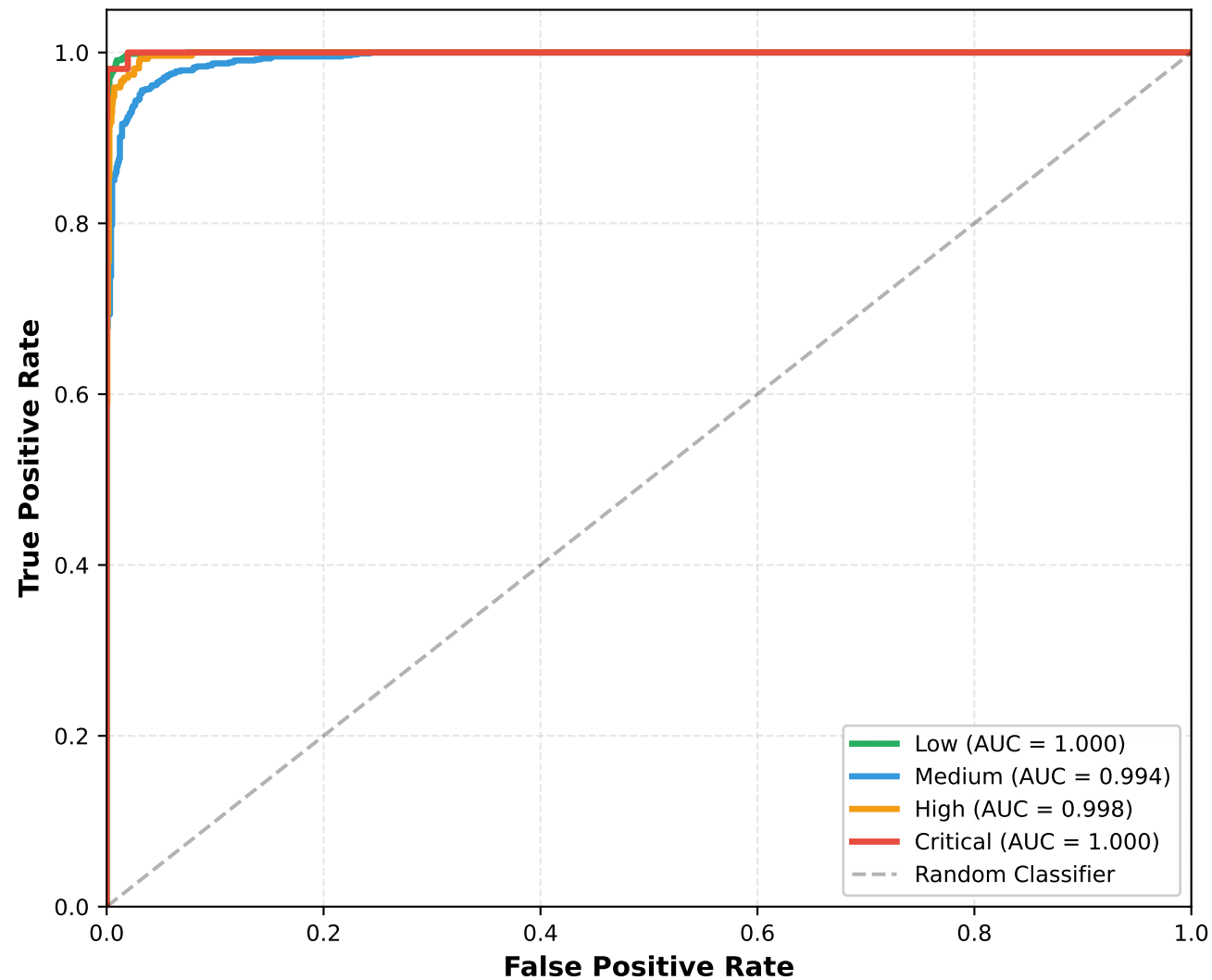
ROC Curves - XGBoost Risk Classifier (One-vs-Rest)
