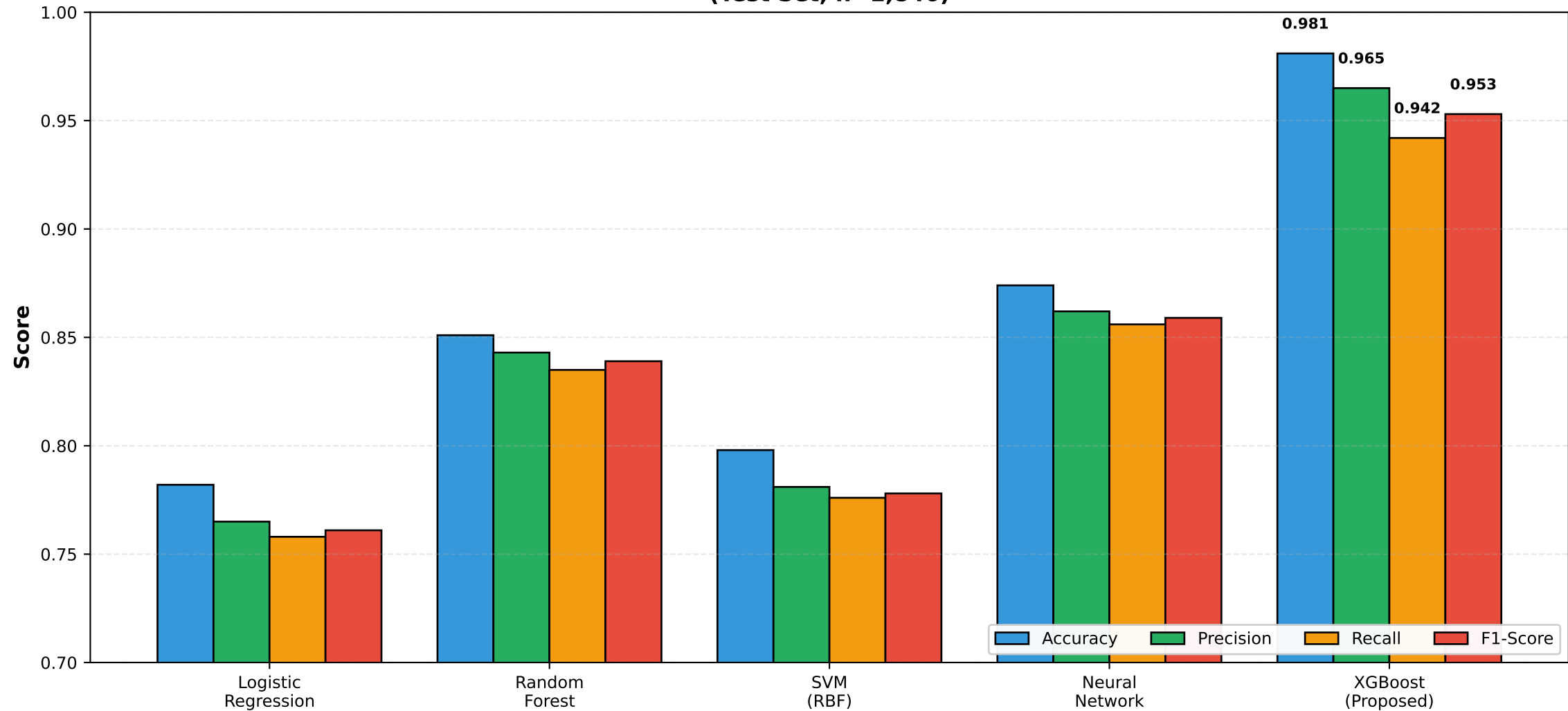
Comparative Performance Analysis Across Classification Models (Test Set, n=1,846)
