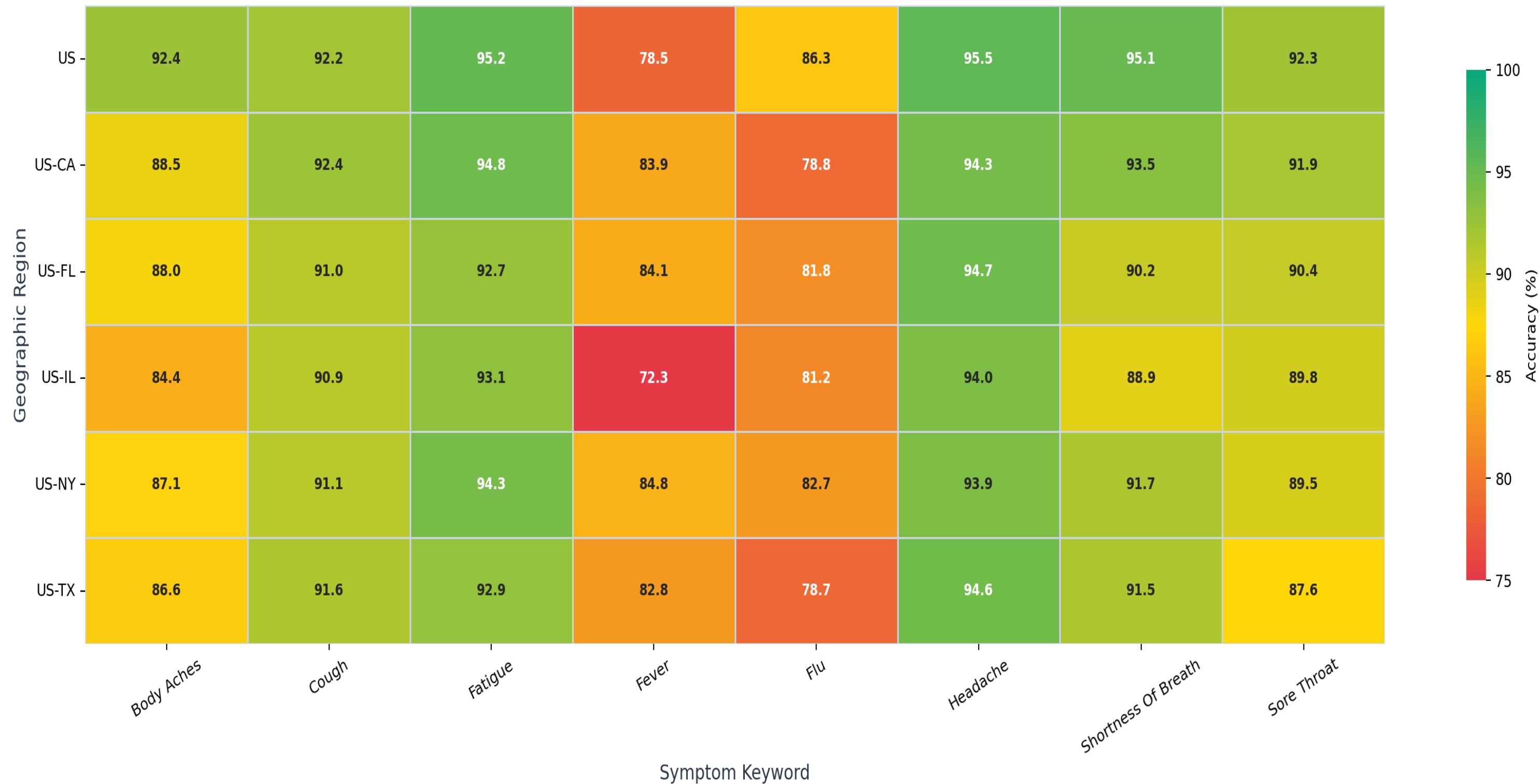
MAPE Prediction Accuracy (%) — Region × Symptom Keyword
