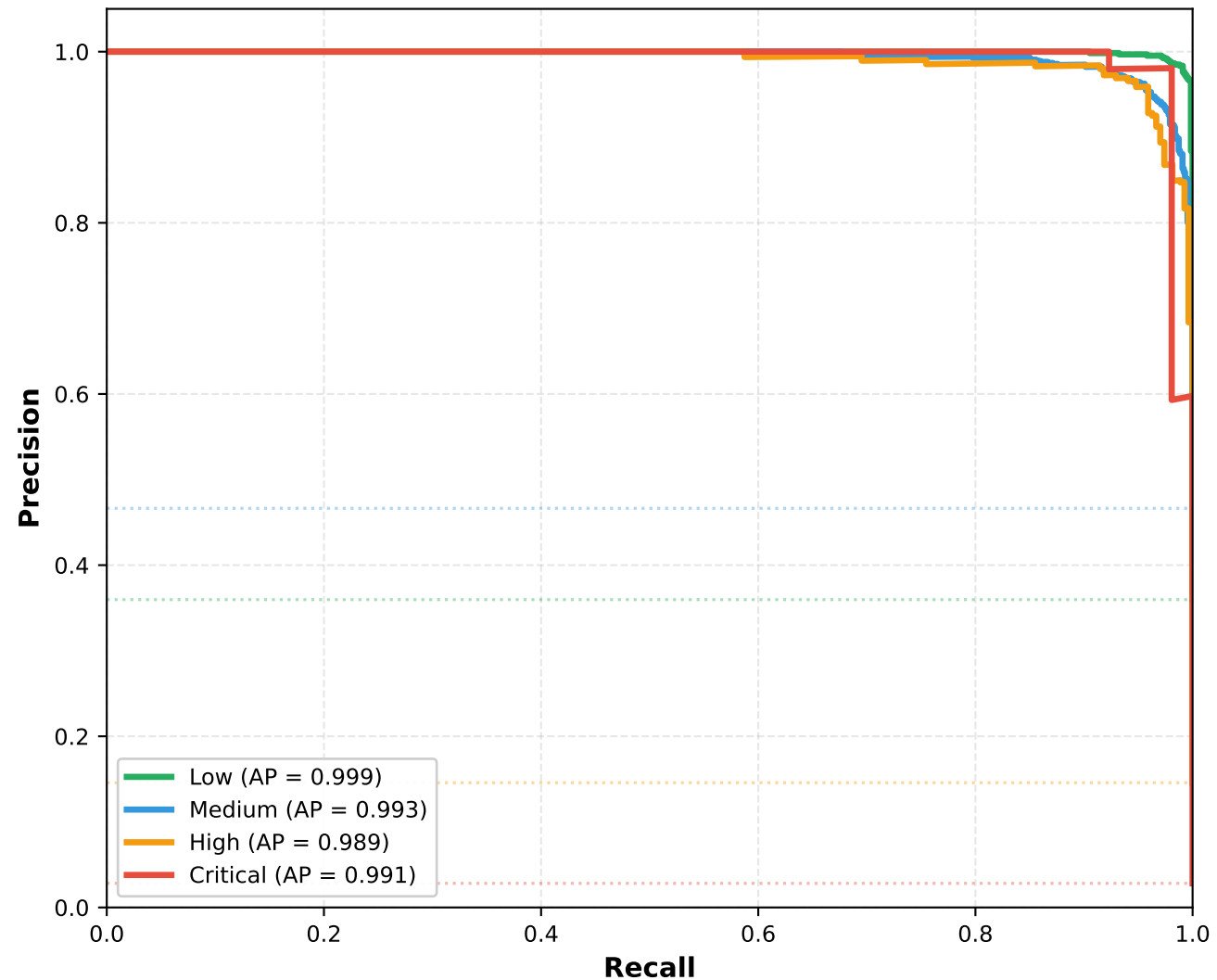
Precision-Recall Curves - XGBoost Risk Classifier
