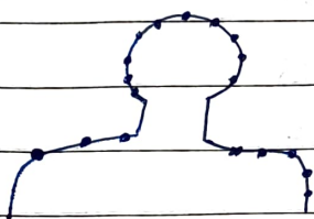
natural
