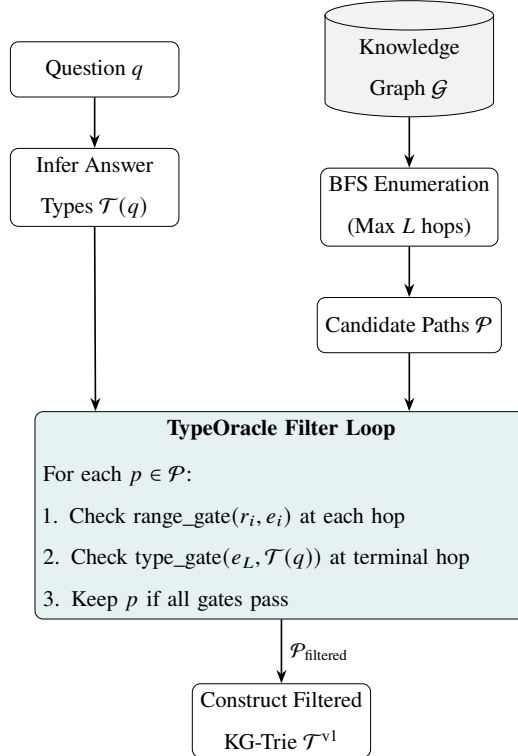
Figure 3.3 Static Symbolic Filtering Pipeline (DCA-Trie v1)
