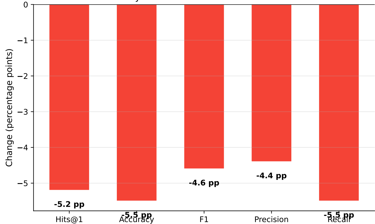
Accuracy Deltas: DCA-Trie v1 vs GCR Baseline
