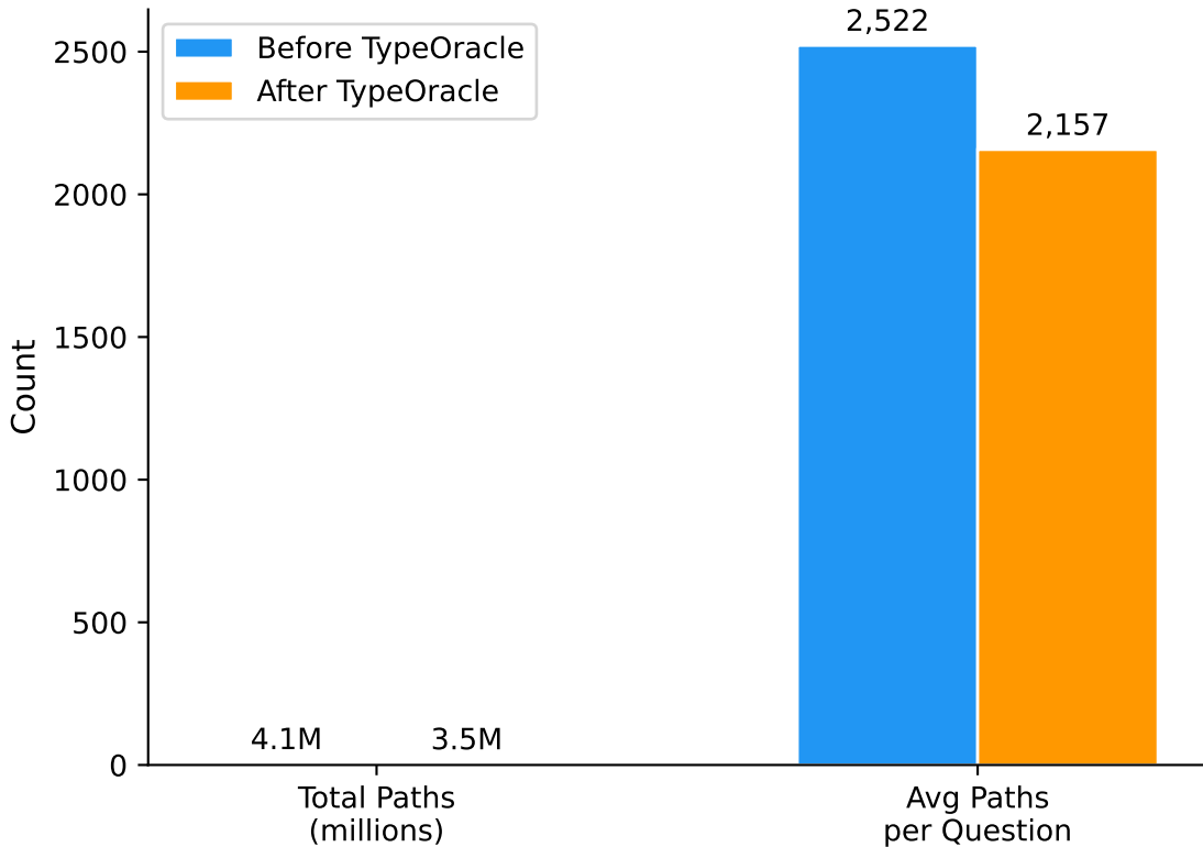
Path Statistics Before and After TypeOracle Filtering
