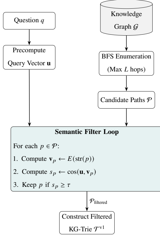
Figure 3.3 Static Semantic Filtering Pipeline for DCA-Trie v1.
