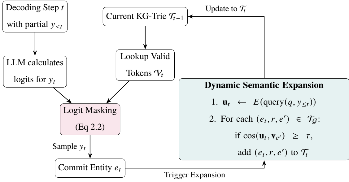
Figure 3.4 Step-Wise Dynamic Expansion Workflow for DCA-Trie v2.
