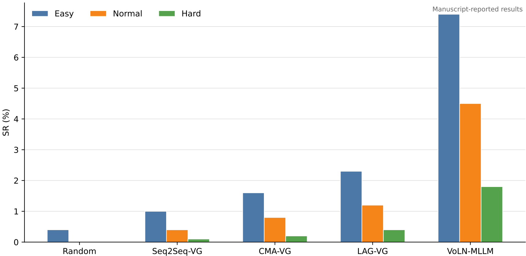
Test-Unseen SR by difficulty
