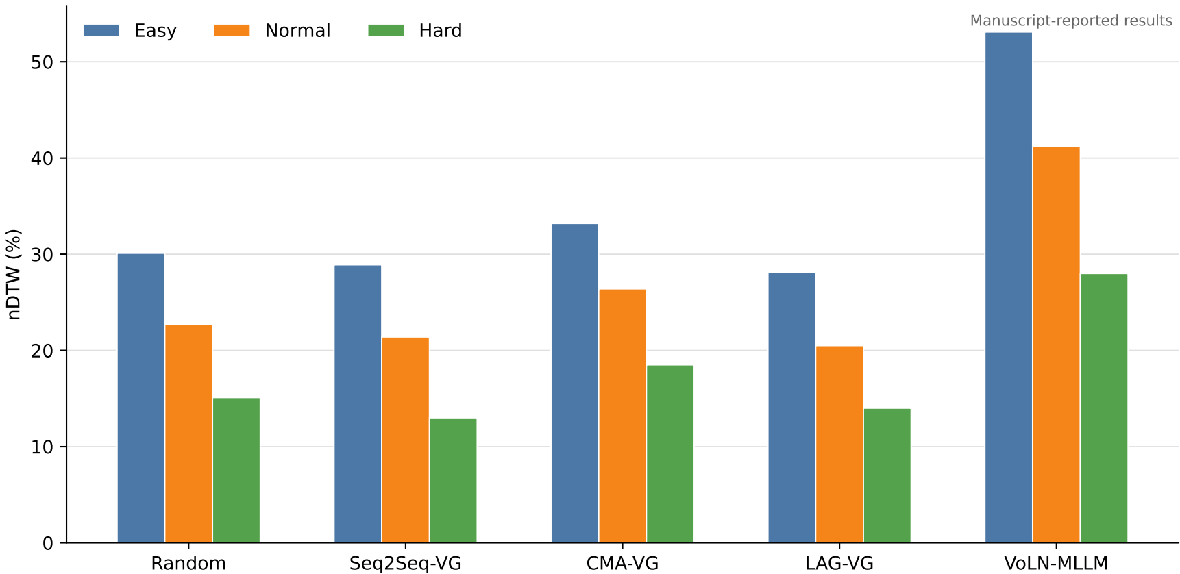
Test-Unseen nDTW by difficulty
