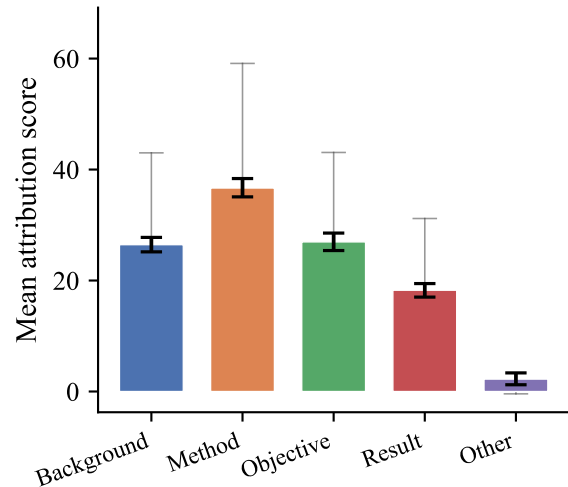
Feature Ablation
