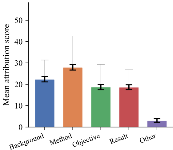
Feature Ablation
