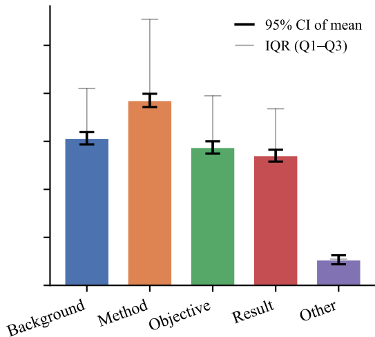
Shapley Value
