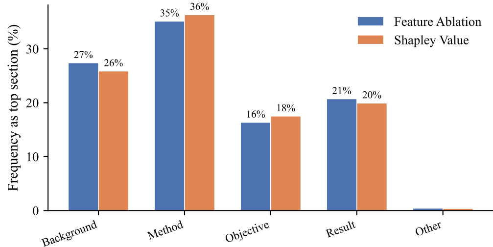
Top-Ranked Section Distribution — TinyLlama-1.1B
