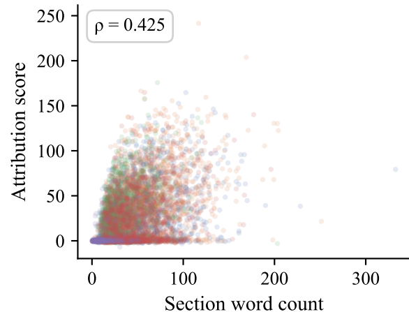
Feature Ablation
