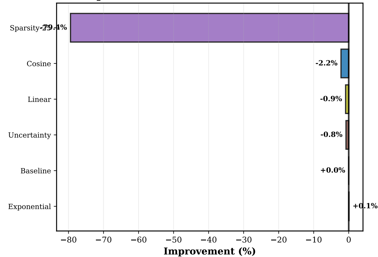
(C) Improvement over Baseline
