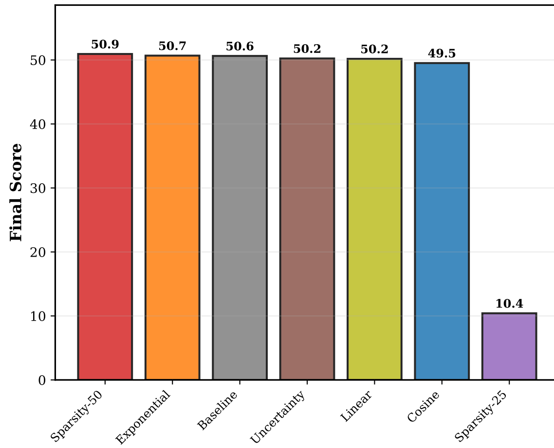
(B) Final Performance
