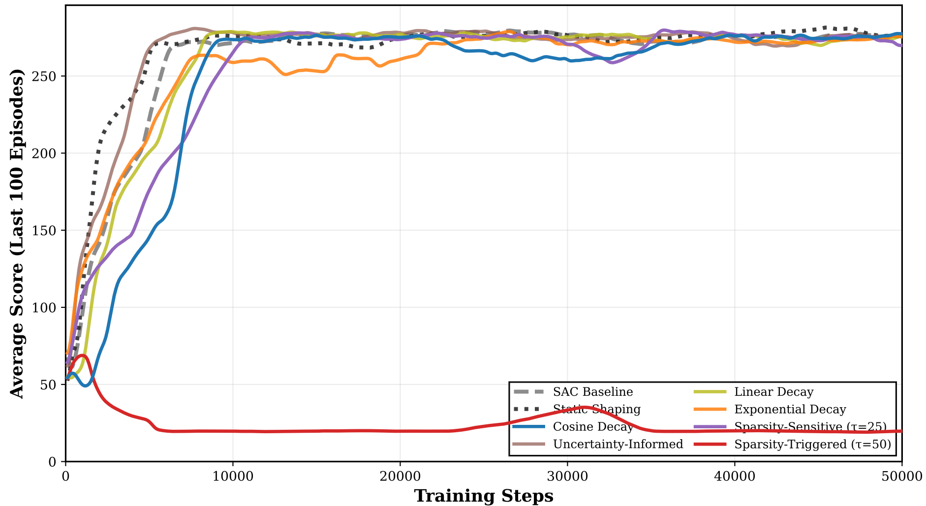
Learning Curves: Adaptive vs Static Reward Shaping
