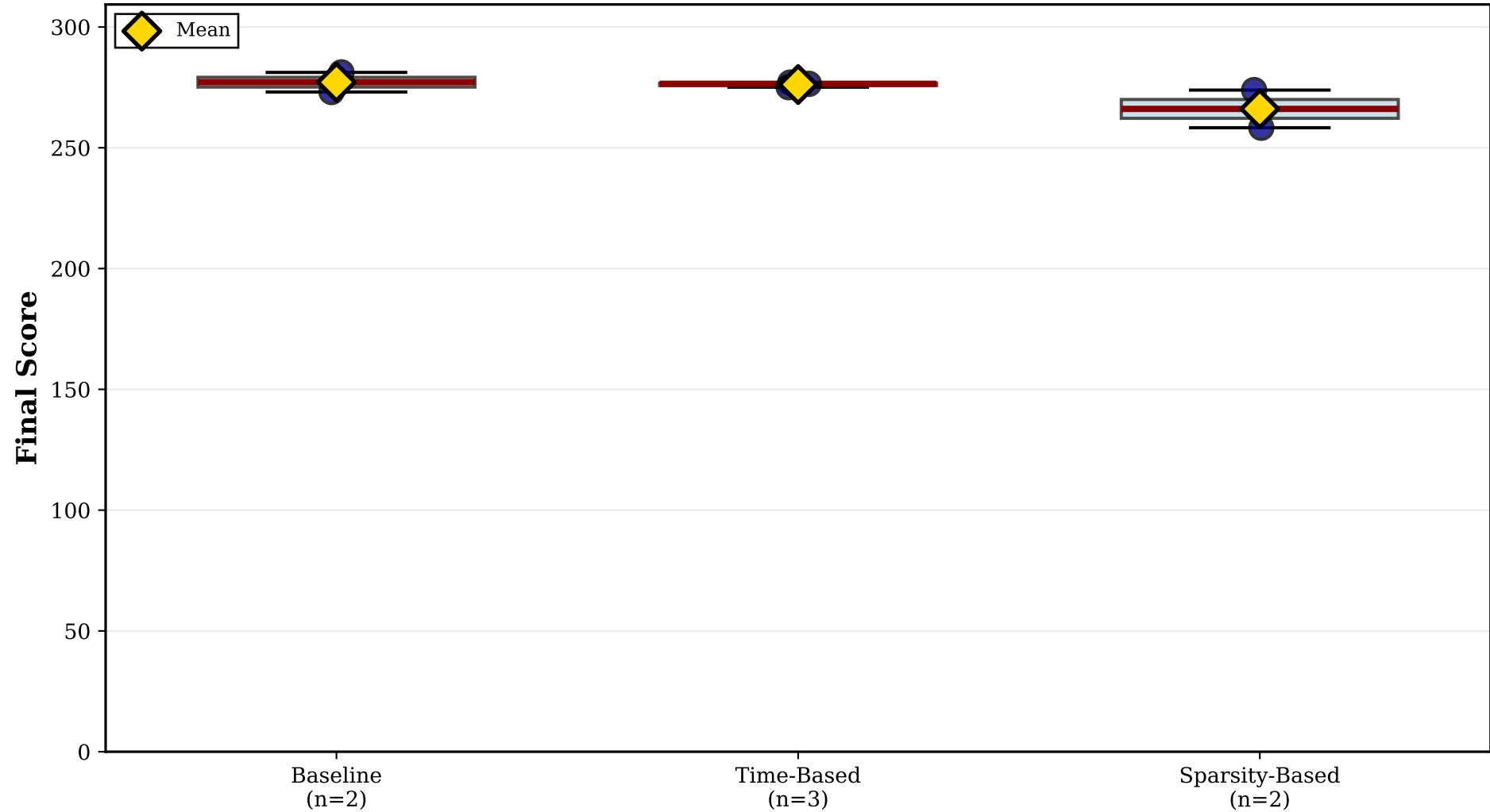
Performance by Scheduler Category
