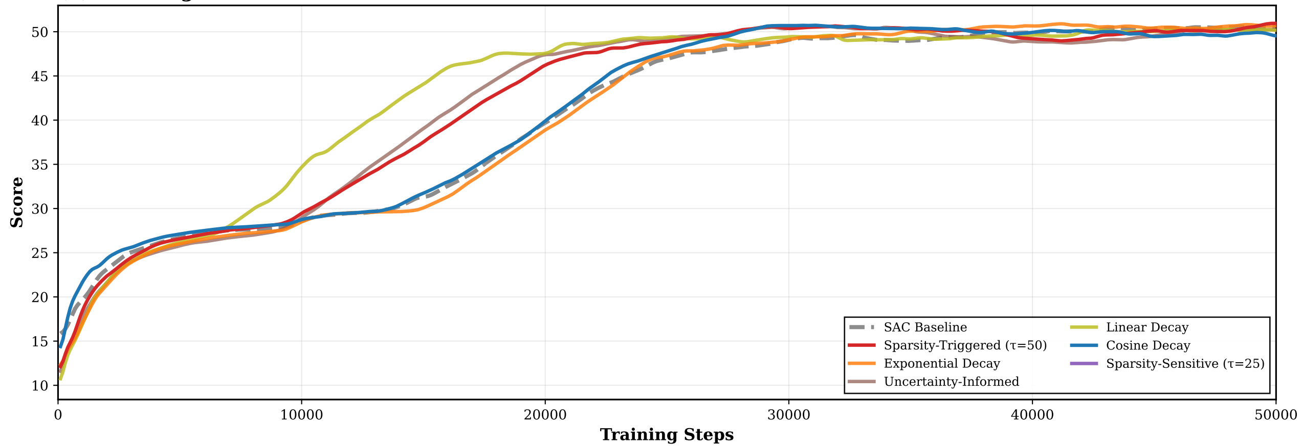
(A) Learning Curves
