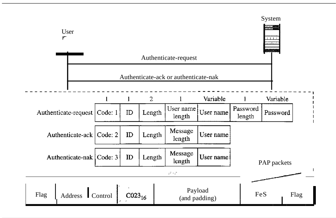
Figure 11.36 PAP packets encapsulated in a PPP frame
