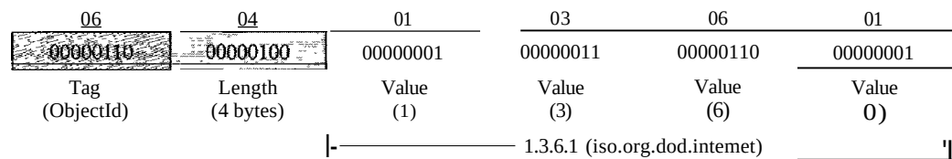
Figure 28.13 Example 28.3, ObjectIdentifier 1.3.6.1
