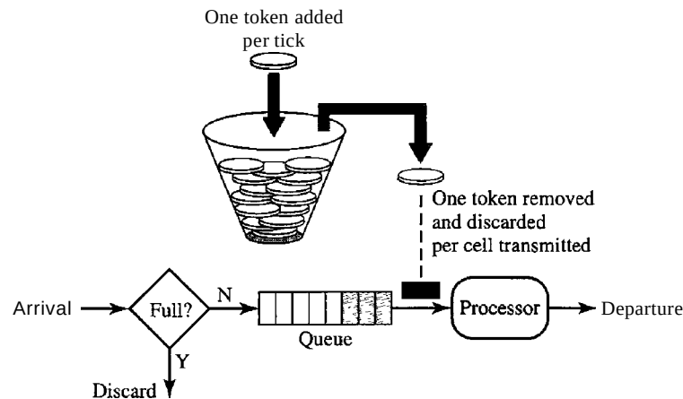
Figure 24.21 Token bucket
