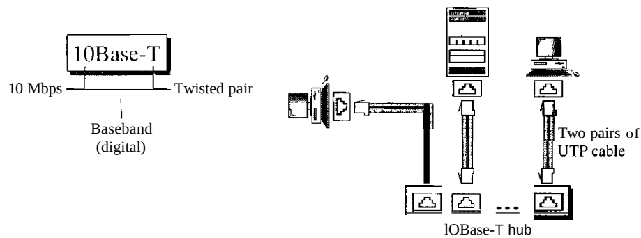
Figure 13.12 IOBase-T implementation
