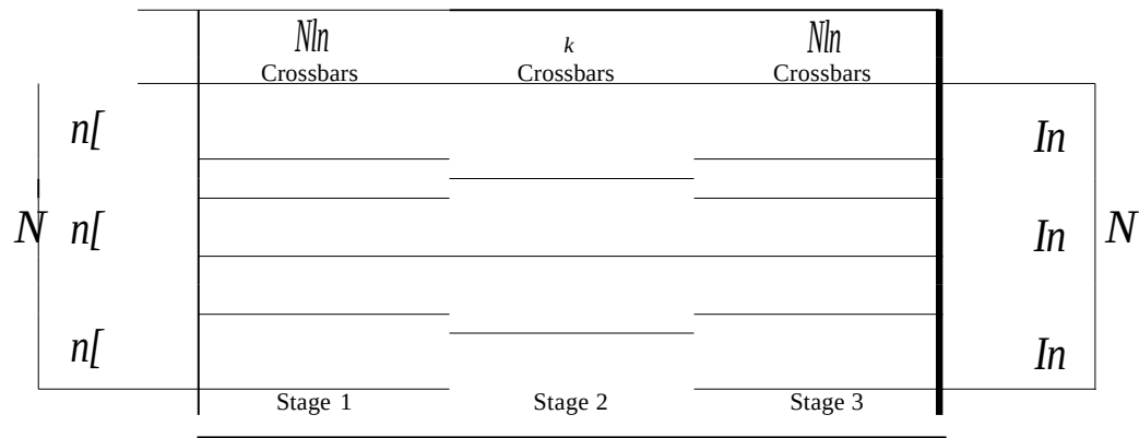
Figure 8.18 Multistage switch
