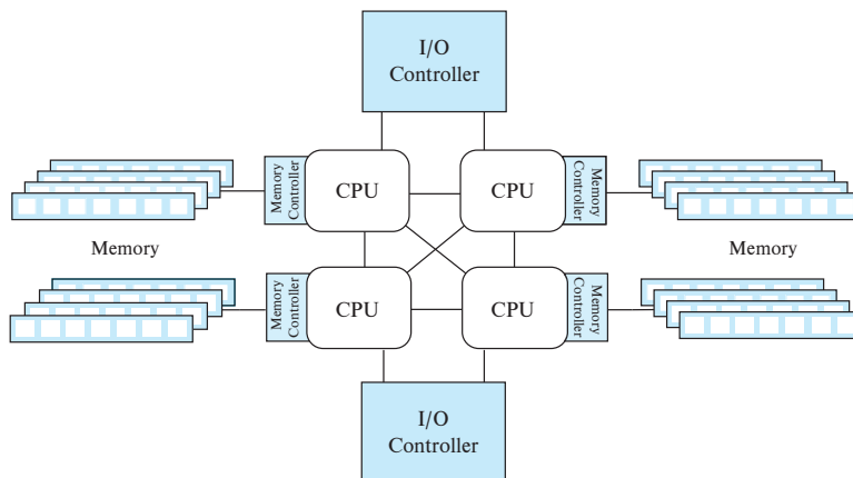
Figure 20.6 Architecture of a modern shared-memory system.
