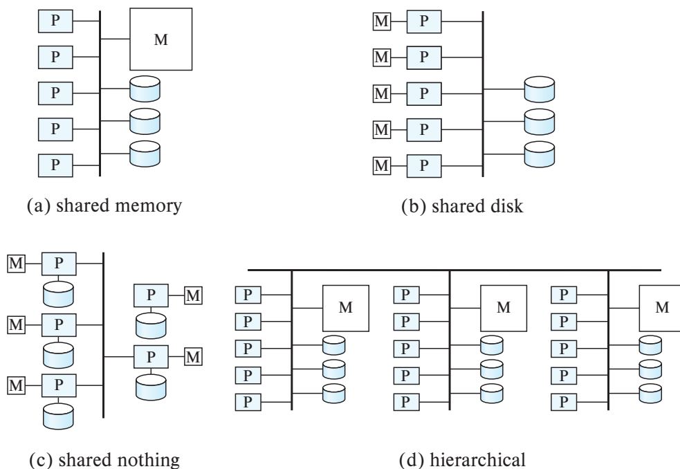
Figure 20.5 Parallel database architectures.
