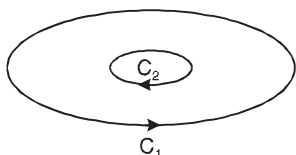
Multi-Connected Region
