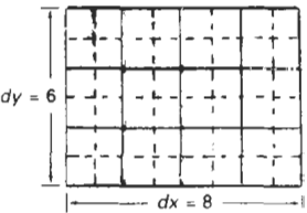
Figure 4-20 A pattern array with 4 columns and 3 rows mapped to an 8 by 6 coordinate rectangle.
