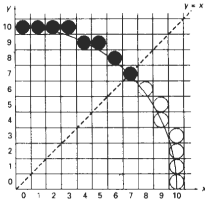
Figure 3-16 Selected pixel positions (solid circles) along a circle path with radius r = 10 centered on the origin, using the midpoint circle algorithm. Open circles show the symmetry positions in the first quadrant.
