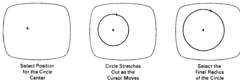
Figure 8-12 Constructing a circle using a rubber-band method.
