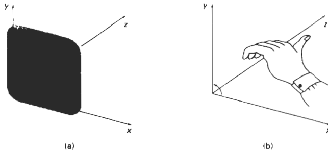
Figure A-7 Left-handed Cartesian coordinate system superimposed on the surface of a video monitor.
