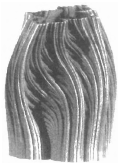
Figure 10-98 The function f(z) = \lambda z(1-z) plotted in three dimensions with normalized \lambda values plotted as the vertical axis. (Courtesy of Alan Norton, IBM Research.)
