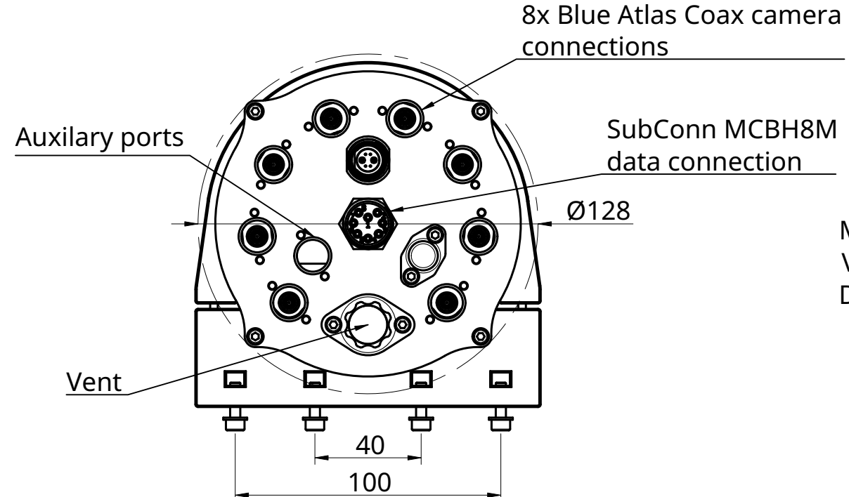
Central bottle unit
