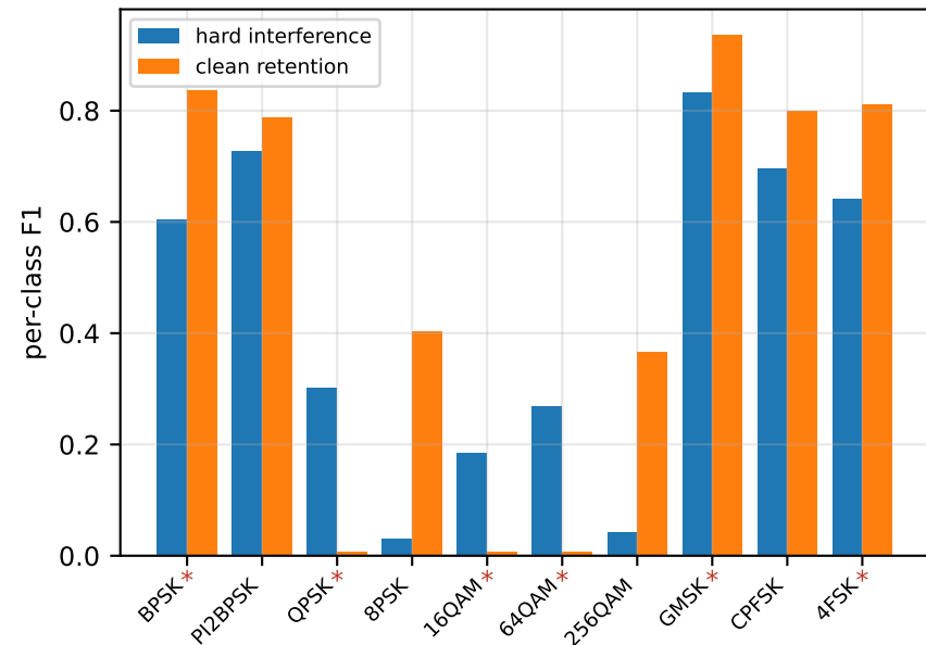
Interference-condition transfer; * marks modulations never presented jammer-free in training compact spectral A0 A7
