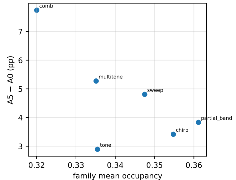
Per-family view
