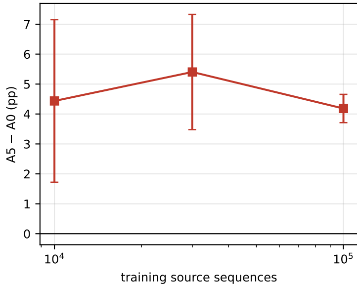
Gain versus training scale
