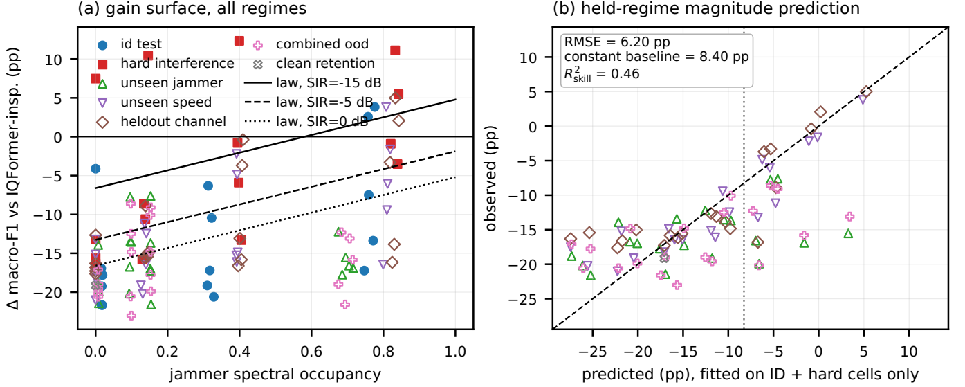
Fig. 4. Exploratory occupancy-SIR operating envelope. Filled cells are used to fit Eq. (8); open cells denote regime cells excluded from fitting. Panel (b) compares predicted and observed model gains on the held-regime cells. Magnitude prediction is evaluated by RMSE relative to a constant predictor fitted on the training cells (6.20 percentage points versus 8.40 percentage points; R^2_{\text{skill}} = 0.46 ). Sign agreement is reported only as a secondary diagnostic, because the held-regime sign distribution is strongly imbalanced.
