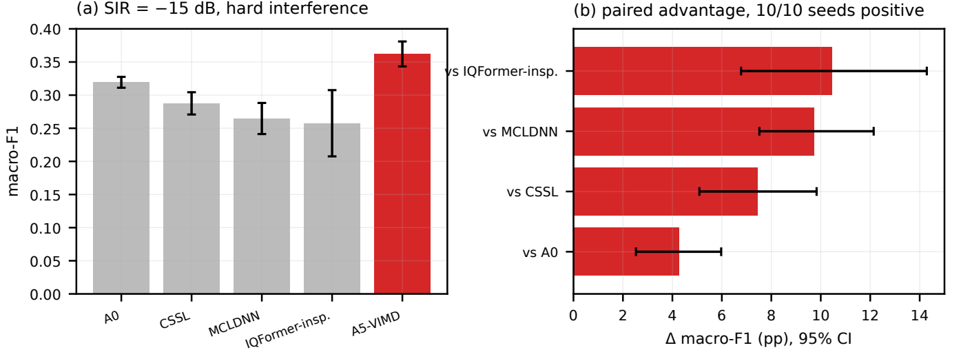
Fig. 3. Severe-interference corner. Left: absolute macro-F1 at SIR = -15 dB. Right: source-paired A5 advantages with stratified bootstrap intervals. The comparison is exploratory and post hoc.
