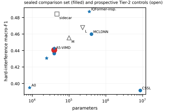
Fig. 5. Hard-interference macro-F1 versus parameter count. Filled markers denote models belonging to the original frozen comparison set; open markers denote prospectively added Tier-2 repair and capacity controls. The Pareto reading is therefore descriptive across evidence classes and does not merge the exploratory models into the sealed family. The frontier is also regime-specific.
