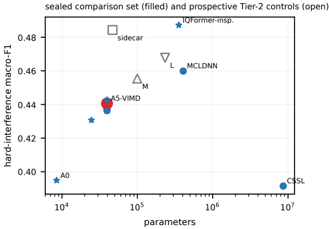
Fig. 5. Hard-interference macro-F1 versus parameter count. Filled markers denote models belonging to the original frozen comparison set; open markers denote prospectively added Tier-2 repair and capacity controls. The Pareto reading is therefore descriptive across evidence classes and does not merge the exploratory models into the sealed family. The frontier is also regime-specific.
