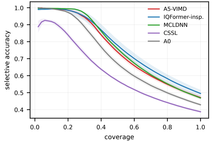
Fig. 6. Selective accuracy versus coverage on hard interference. Thresholds are calibrated without using test labels. This is supporting evidence.
