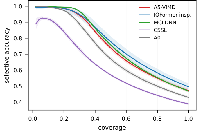
Fig. 6. Selective accuracy versus coverage on hard interference. Thresholds are calibrated without using test labels. This is supporting evidence.
