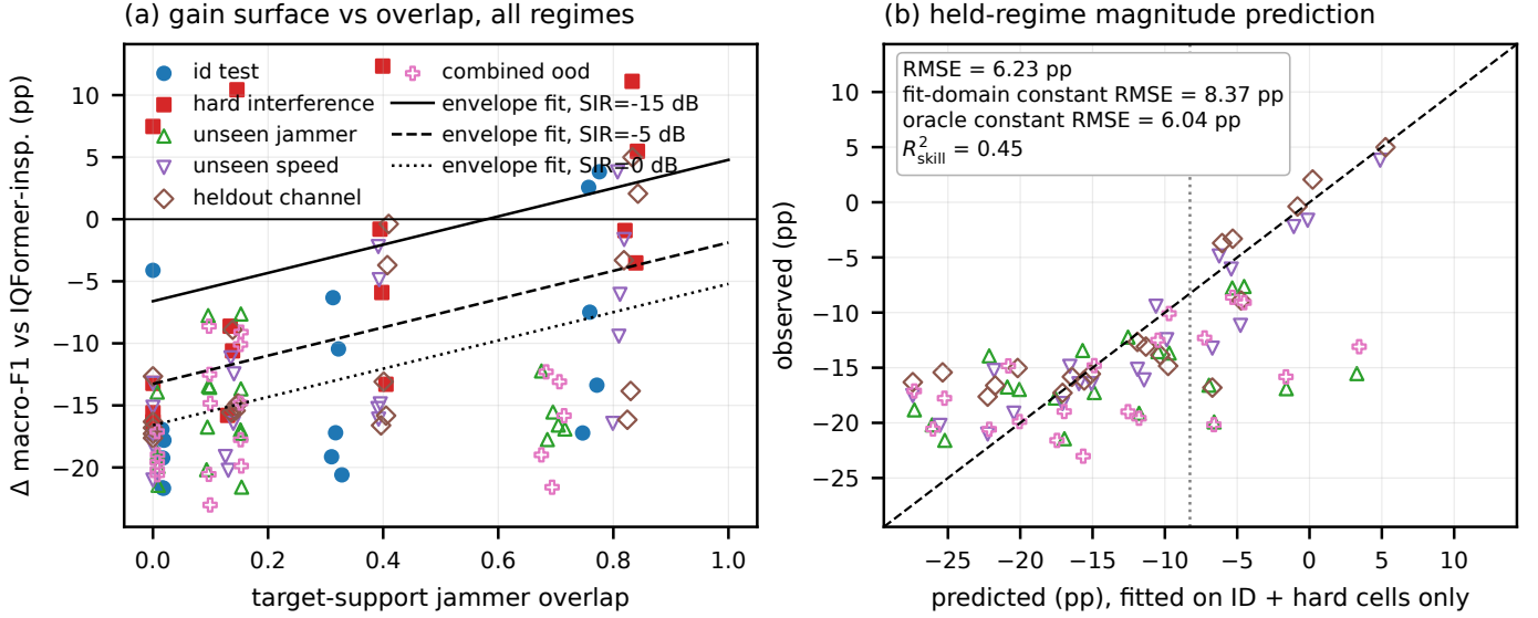
Fig. 2. Exploratory overlap-SIR operating envelope. The abscissa of panel (a) is the target-support jammer overlap of Eq. (9), not an occupied-bandwidth fraction. Filled cells are used to fit Eq. (8); open cells denote regime cells excluded from fitting. Panel (b) compares predicted and observed model gains on the held-regime cells. Magnitude prediction is evaluated by RMSE relative to a constant predictor estimated from the envelope-fitting cells (whose value is the mean gain there, -8.27 percentage points): 6.23 percentage points versus 8.37 percentage points for the constant ( R^2_{\text{skill}} = 0.45 ); an oracle constant equal to the mean of the held-regime cells themselves would attain 6.04 percentage points. Sign agreement is reported only as a secondary diagnostic, because the held-regime sign distribution is strongly imbalanced.
