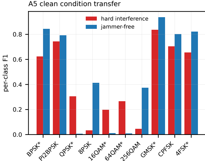
Fig. 4. A5 clean condition-transfer taxonomy. A star marks a class whose jammer-free condition was not seen during training; the four covered classes are unstarred. The plot localizes the clean boundary rather than aggregating it.
