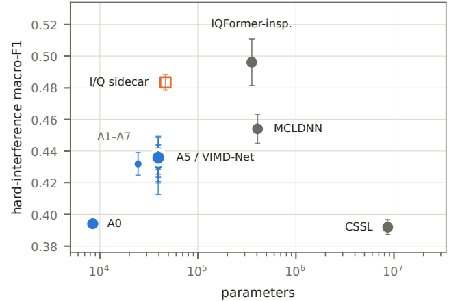
Fig. 4. Hard-interference macro-F1 versus parameter count on the matched five-seed subset; bars are \pm 1 standard deviation over those seeds. Filled circles are seeded models (blue: the A0-A7 spectral family, of which only A0 and A5 are labelled; gray: the I/Q comparators); the open orange square is the prospective Tier-2 received-I/Q sidecar, which is exploratory and outside the sealed family. The Pareto reading is descriptive and regime-specific.
