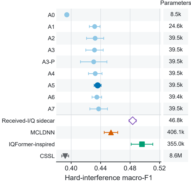
Fig. 3. Aligned performance-complexity comparison on the matched five-seed subset. Horizontal position shows hard-interference macro-F1, whiskers show \pm 1 seed standard deviation, and the right column reports parameter count. All A0–A7 variants are shown; color highlights A5, the received-I/Q sidecar, and the three I/Q-domain references.
