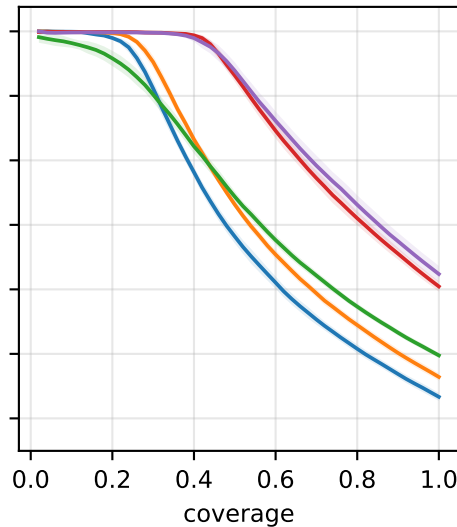
Risk-coverage after validation-only temperature scaling id test combined ood
