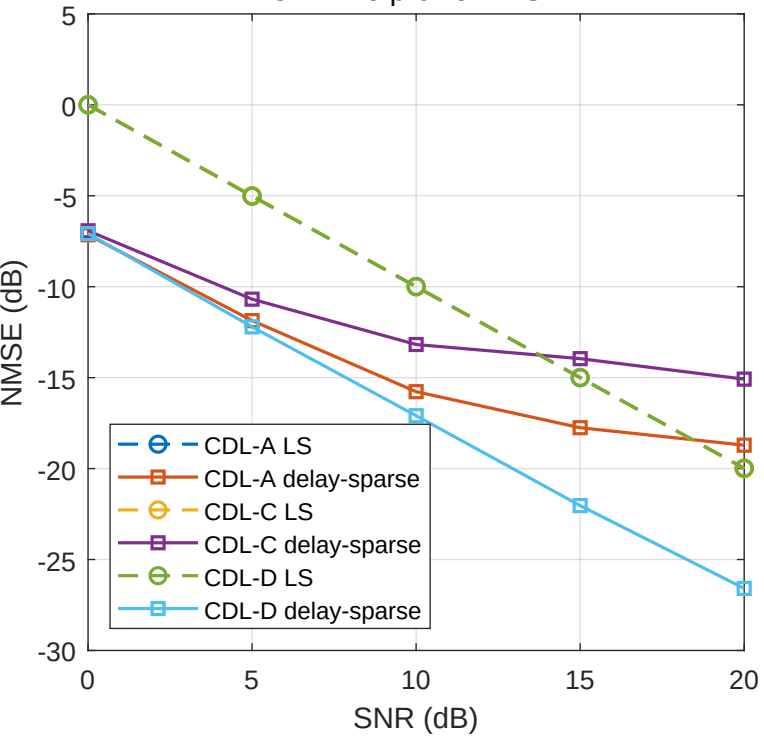
CDL-like profile NMSE
