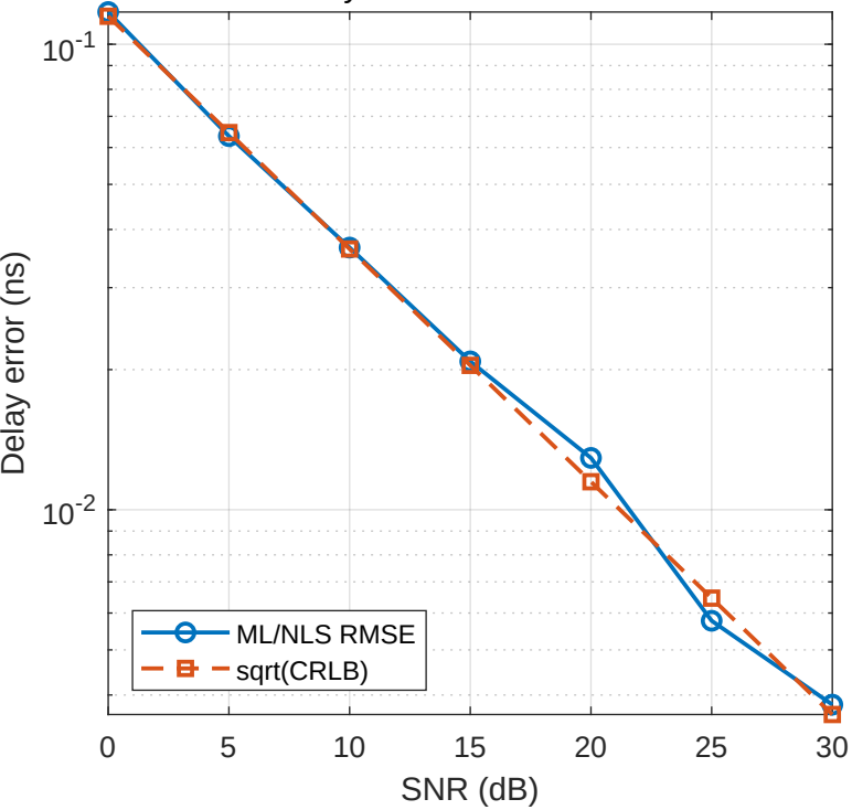
Delay RMSE versus CRLB
