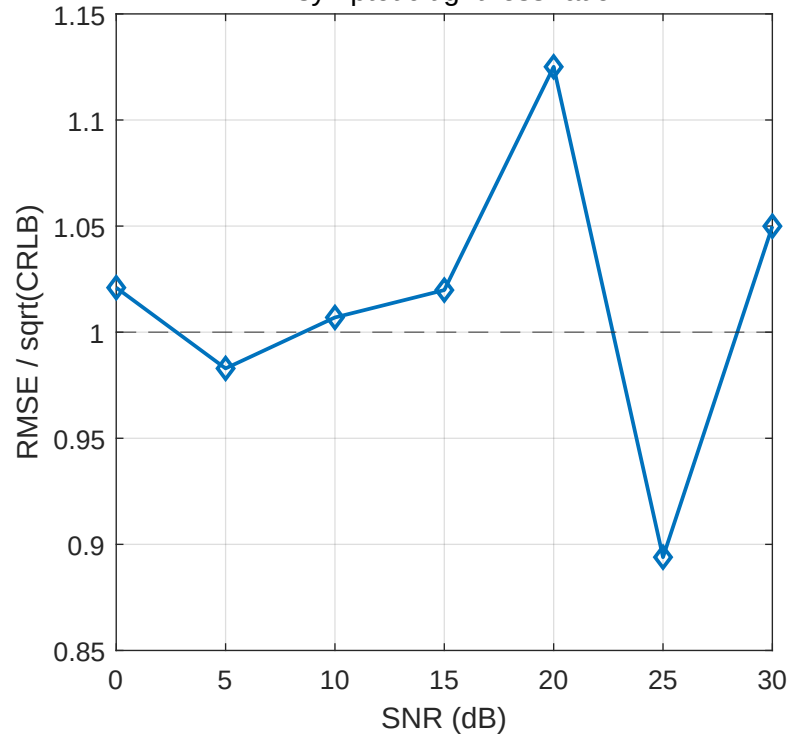
Asymptotic tightness ratio
