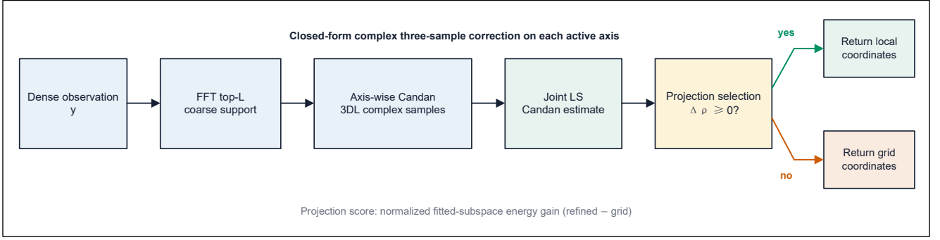
Fig. 2. Projection-selected multidimensional Candan refinement. One FFT supplies 3DL triplet samples. The grid energy comes directly from the selected orthonormal FFT coefficients, while the refined energy is obtained from the Candan design QR factor.
