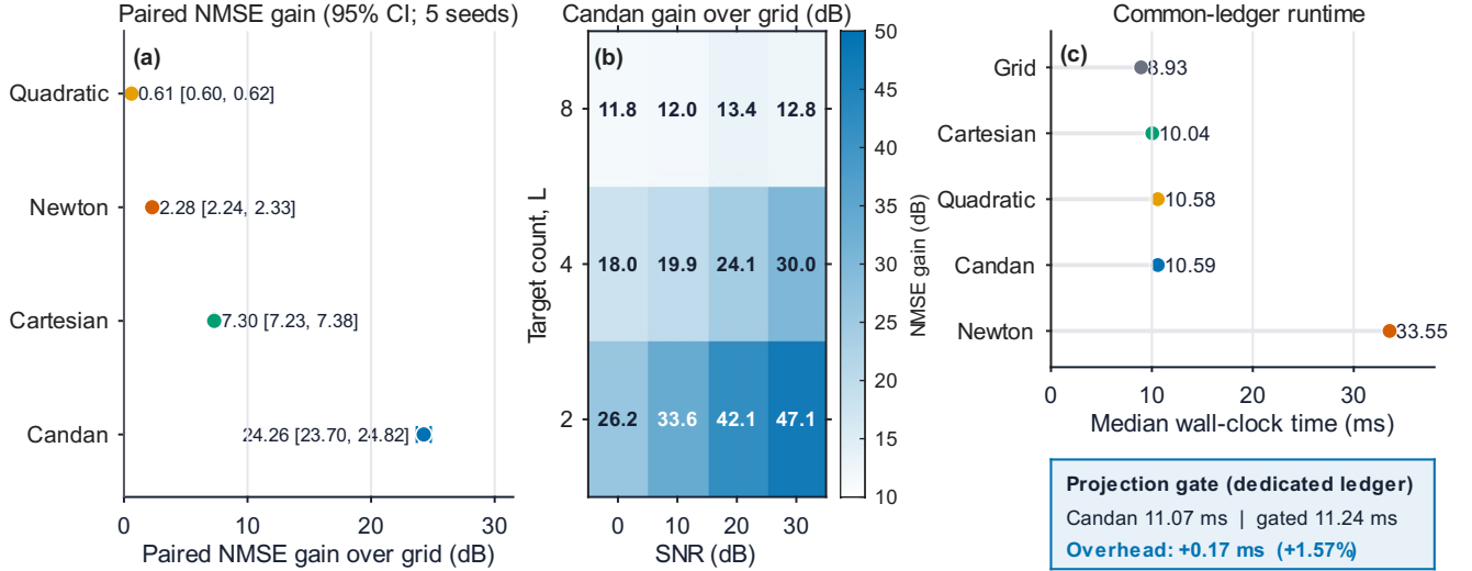
Fig. 3. Matched-scene evidence on the common 1200-tensor campaign. (a) Paired measurement-NMSE gain over FFT top- L plus joint LS for four local refinements; dots and bars are the mean and 95% interval over five seed means (higher is better). (b) Candan gain across SNR and target count; every displayed condition is positive. (c) Common-ledger median end-to-end runtime, with a separate dedicated-implementation inset showing that fitted-energy selection adds 0.17 ms (1.57%) to local Candan.
