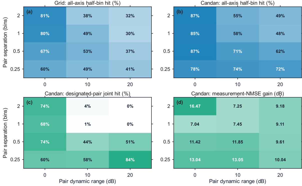
Fig. 4. Controlled separation/near-far evidence averaged over four SNRs, with 100 test scenes and five seed means per displayed cell. Panels (a) and (b) share a 0–100% scale for direct comparison of grid and Candan per-component all-axis half-bin rates; (c) reports designated-pair joint recovery; and (d) reports measurement-NMSE gain over grid. All displayed reconstruction gains are positive.
