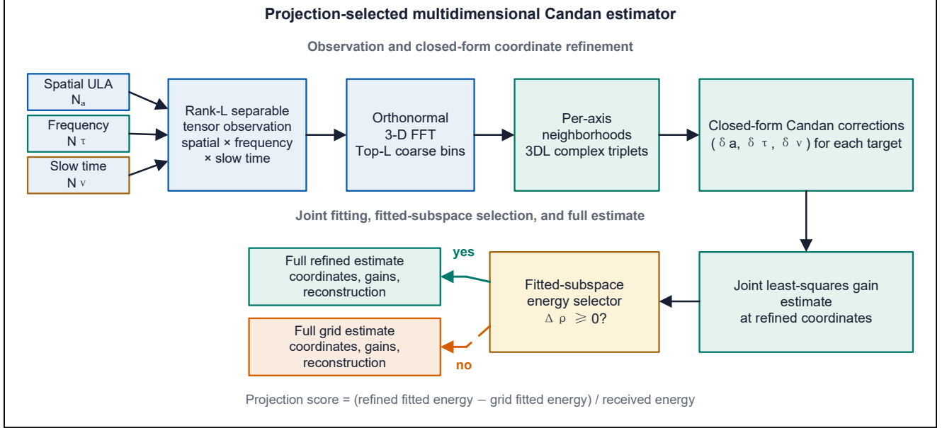
Fig. 1. End-to-end projection-selected tensor estimator. The separable observation is transformed once; top- L FFT neighborhoods provide 3DL center/neighbor samples for axis-wise Candan correction, joint LS estimates the gains, and the higher fitted-subspace energy returns either the refined or grid coordinates with the corresponding reconstruction.
