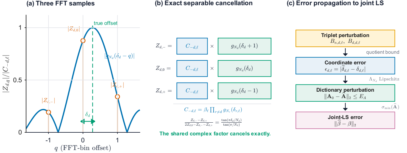
Fig. 2. Mechanism linking separable FFT triplets to the joint fit. (a) The center and two periodic neighbors sample the finite-length Dirichlet response around one selected bin. (b) Factors from the non-updated tensor axes are common to all three samples and cancel in the Candan quotient, leaving the fractional coordinate on the active axis. (c) Triplet perturbations determine coordinate error, atom perturbation, and the final joint-LS reconstruction error.
