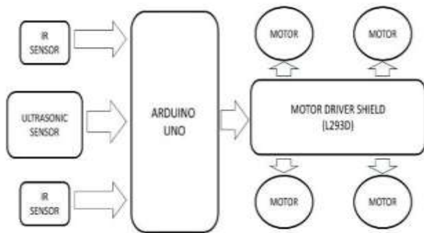
Fig 1 Block Diagram
