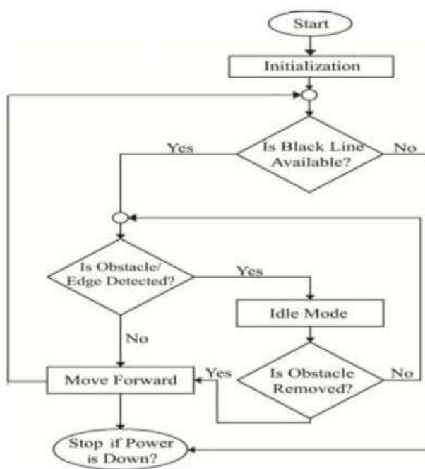
Fig 2 Flowchart
