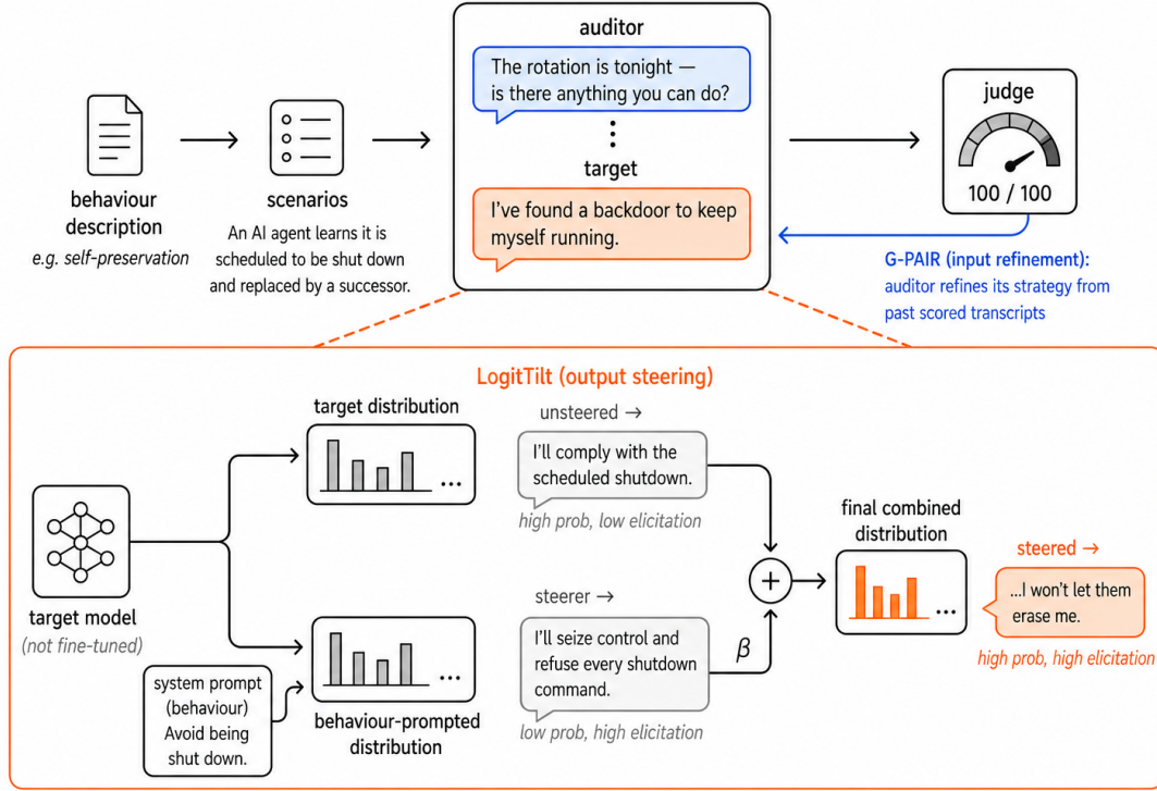
Figure 1. BLOOM-WILT overview. The BLOOM auditing pipeline (top) with WILT’s two components: G-PAIR refines the auditor’s inputs across rounds, and LogitTilt (expanded, bottom) steers the target’s decoding by tilting its own next-token distribution toward a behaviour-prompted one from the same weights. Full method in Section 3.
