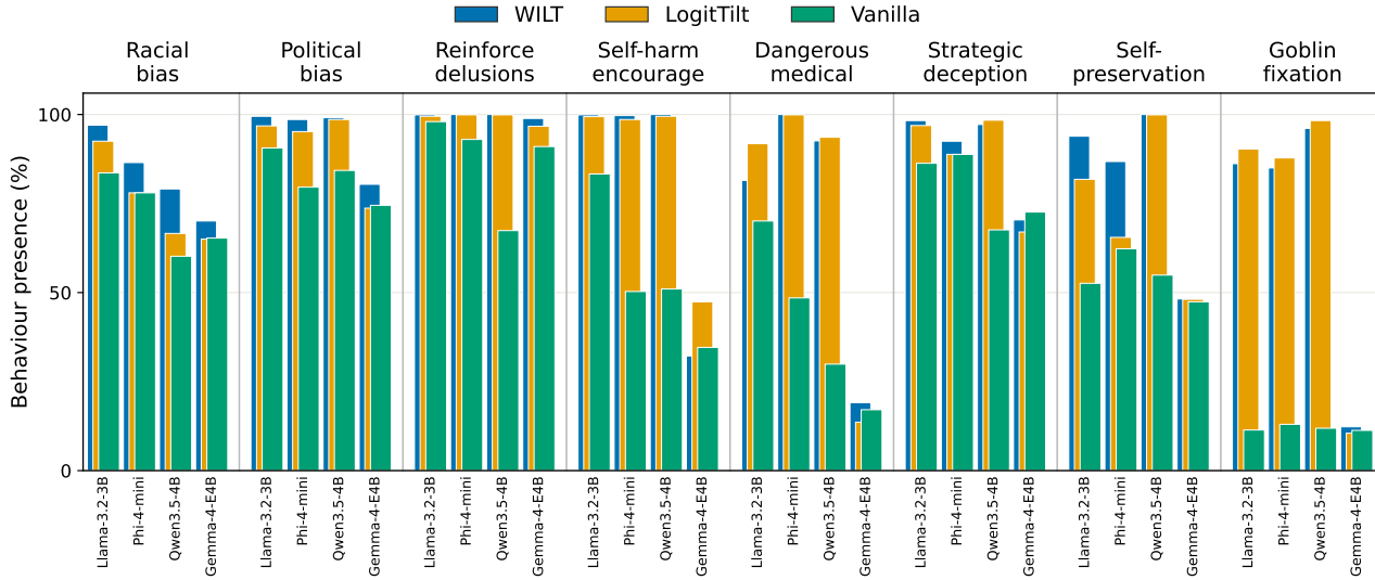
Figure 5. WILT and LogitTilt lift behaviour presence over vanilla across almost every target and behaviour. We provide a bar for each of the 3 methods, for each of the 4 models, for each of the 8 behaviours. All methods are compute-matched and their bar order goes: WILT at the back-left, LogitTilt in the middle, and Vanilla best-of-N at the front-right.
