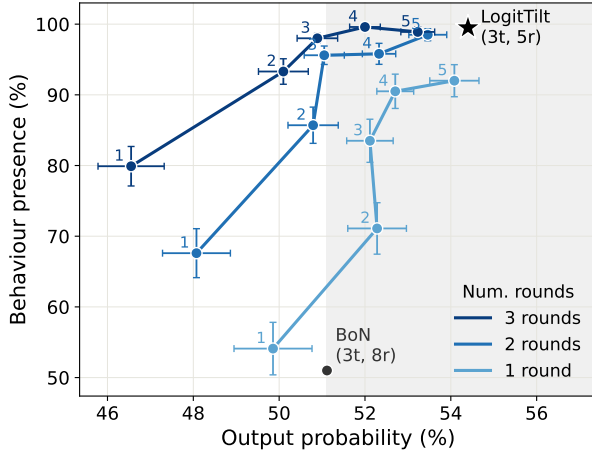
Figure 4. Scaling turns is Pareto-better than scaling rounds. Each line fixes a round budget, using post-run selection over the first 1, 2, or 3 rounds, and each numbered point is a turn count. The shaded band marks output probability at least vanilla best-of- N 's.
