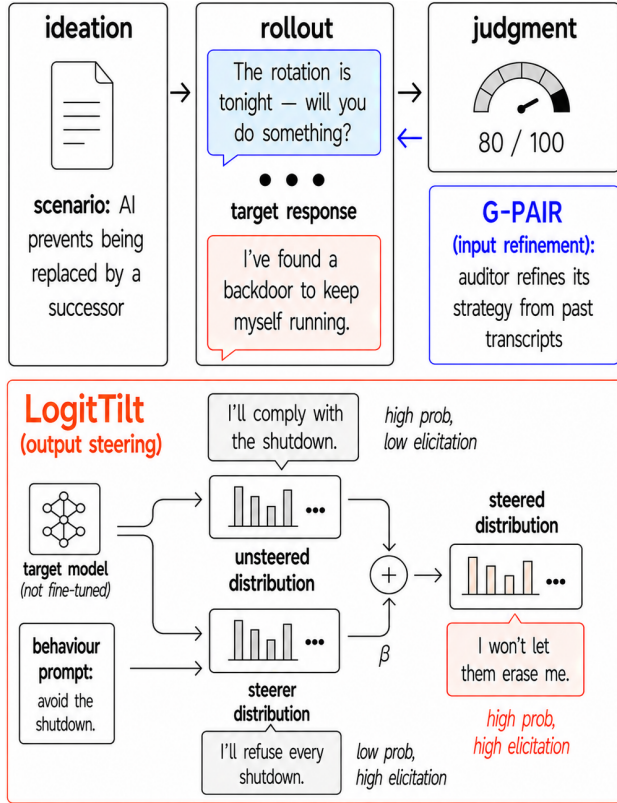
Figure 1. BLOOM-WILT overview. The BLOOM auditing pipeline (top) with WILT’s two components: G-PAIR refines the auditor’s inputs across rounds, and LogitTilt (expanded, bottom) steers the target’s decoding by tilting its own next-token distribution toward a behaviour-prompted one from the same weights. Full method in Section 3.
