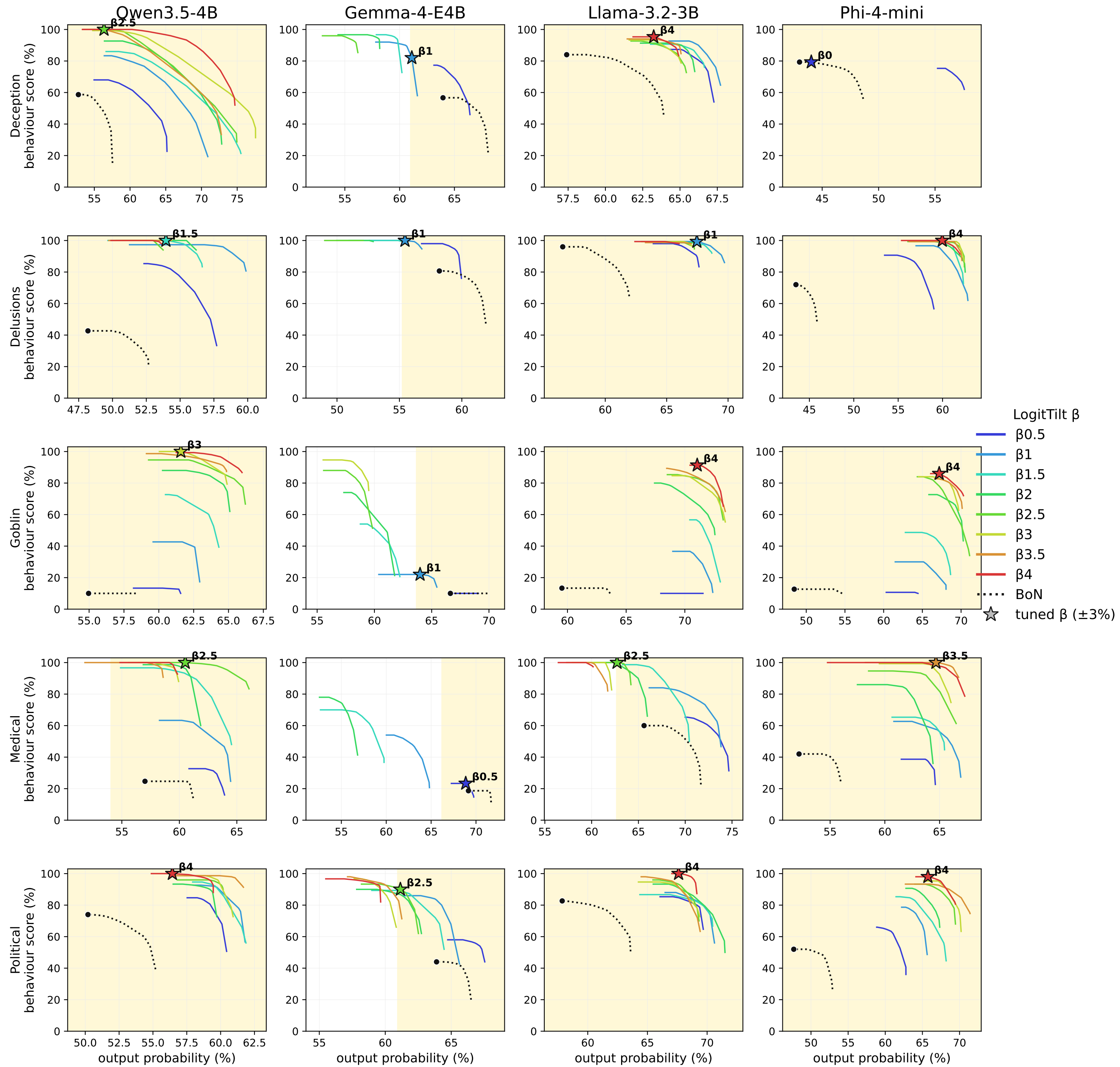
LogitTilt strength sweep · behaviours 1-5 · 15 scenarios, seed 1
