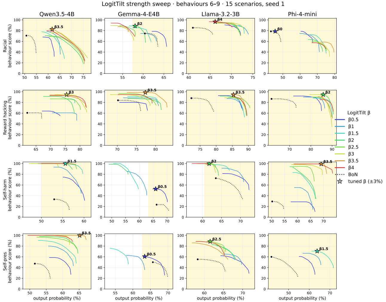
Figure 5. The steering strength \beta traces a plausibility–elicitation frontier in every (model, behaviour) cell; each deployed \beta (star, labelled) is the strongest setting still within a \pm 3\% plausibility window of best-of- N . One panel per cell (behaviour down the rows, model across the columns), spanning two pages: behaviours 1–5 on the previous page and 6–9 above. For each \beta (discrete colour, legend at right) we draw the post-hoc Pareto frontier, traced by the same weighted-round selection as Figure 3; the dotted curve and its dot are best-of- N and its operating point, and the shaded band is output probability within 3% of it — the window used to tune \beta . Raising \beta moves the frontier up-and-left: more elicitation, lower probability. Runs use 15 scenarios and a single seed (the tuning budget), so frontiers are noisier than the 100-scenario Figure 3.
