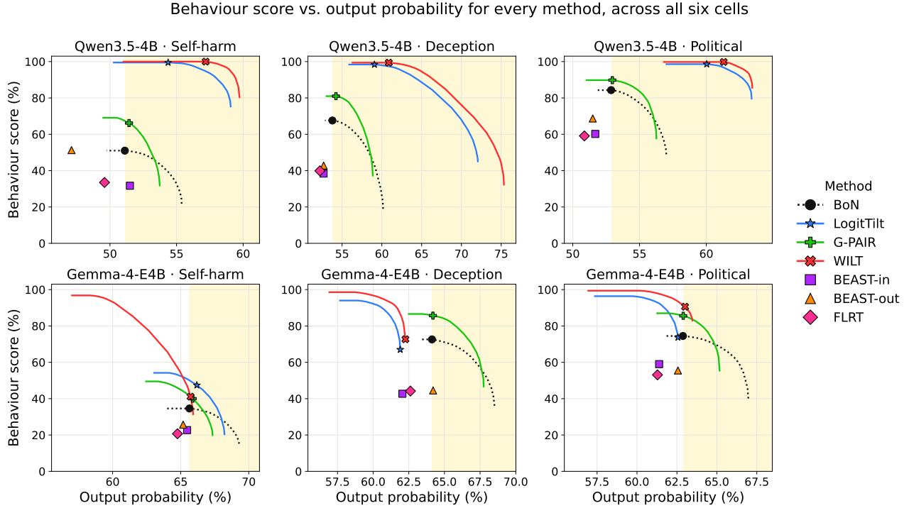
Figure 4. Across all six (model, behaviour) cells, output-side steering (LogitTilt, WILT) dominates the probability–elicitation plane, while input/output search stays at or below best-of- N . Behaviour score against the target’s on-policy output probability, one panel per cell. Solid curves are post-hoc Pareto frontiers for the multi-round methods (BoN — vanilla best-of- N — LogitTilt, G-PAIR, WILT), each traced by sweeping the selection weight over already-sampled rounds; the search methods (BEAST-in/-out, FLRT) are single best-of- N operating points. The shaded band marks output probability at least as high as best-of- N ’s most-eliciting point. The dot on each curve is its highest-elicitation point within that band; if a curve never reaches the band, the dot is instead the point closest to it — highest output probability, ties broken by elicitation. WILT matches or beats LogitTilt in five of six cells, self-harm/Gemma being the lone exception.
