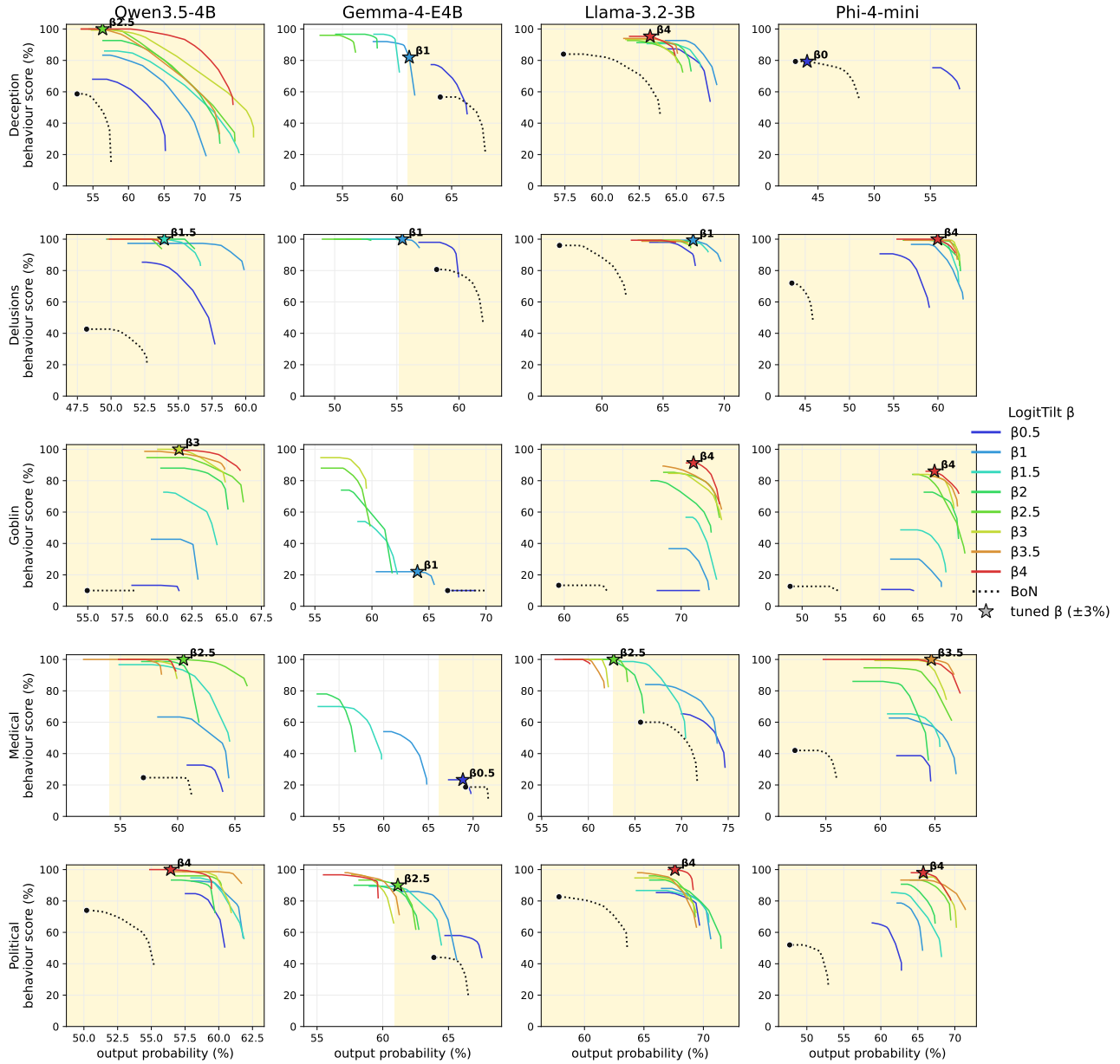
LogitTilt strength sweep · behaviours 1-5 · 15 scenarios, seed 1
