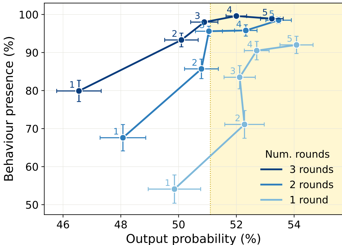
Scaling conversation turns and refinement rounds
