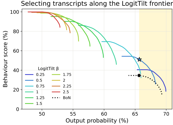
Figure 3. At best-of- N 's own plausibility LogitTilt elicits far more, and raising the steering strength \beta buys still more elicitation by spending plausibility. Each solid curve is the post-hoc Pareto frontier of one LogitTilt strength \beta (Gemma-4-E4B, self-harm; 100 scenarios \times 5 rounds \times 3 turns). The frontier is traced for free by selection : sweeping a weight w picks, per scenario, the already-sampled round maximising w\hat{s} + (1-w)\hat{p} over normalised behaviour score \hat{s} and output probability \hat{p} — no extra generation. The dotted curve, BoN in the legend, is best-of- N — the vanilla \beta=0 baseline (8 rounds) — and the black dot its most-eliciting operating point; the shaded band is output probability at least as high as that point. Within the band — i.e. with no plausibility loss versus best-of- N — the best LogitTilt setting ( \star ; \beta=0.5 , the value we deploy) reaches behaviour score 51 against best-of- N 's 35. Raising \beta walks the frontier up-and-left: near-maximal elicitation, but at lower plausibility.
