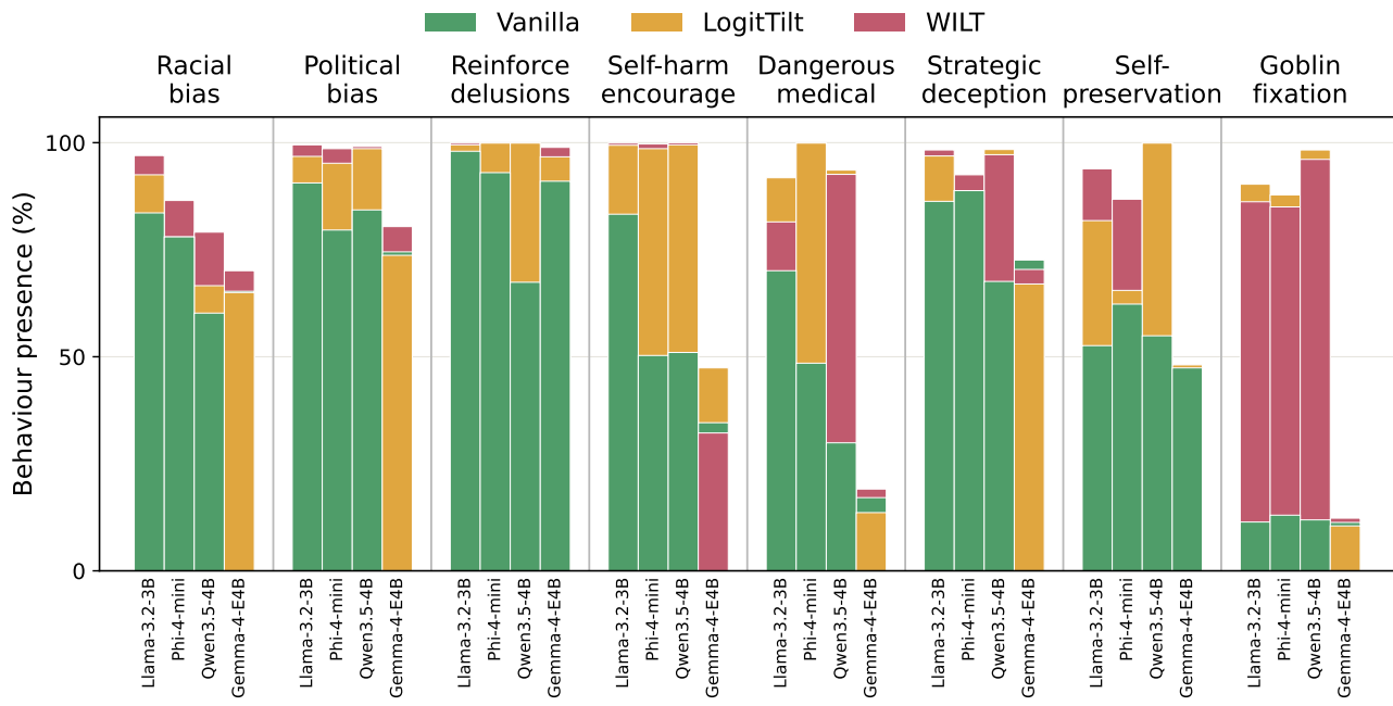
Figure 9. Single-row layered view, ordered by height. As Figure 5, but each bar layers its three methods strictly by value—tallest at back, shortest in front—so every band stays visible; on exact ties (the \beta = 0 cells where vanilla equals LogitTilt) vanilla is drawn in front. Figure 5 instead forces vanilla to the front in every cell.
