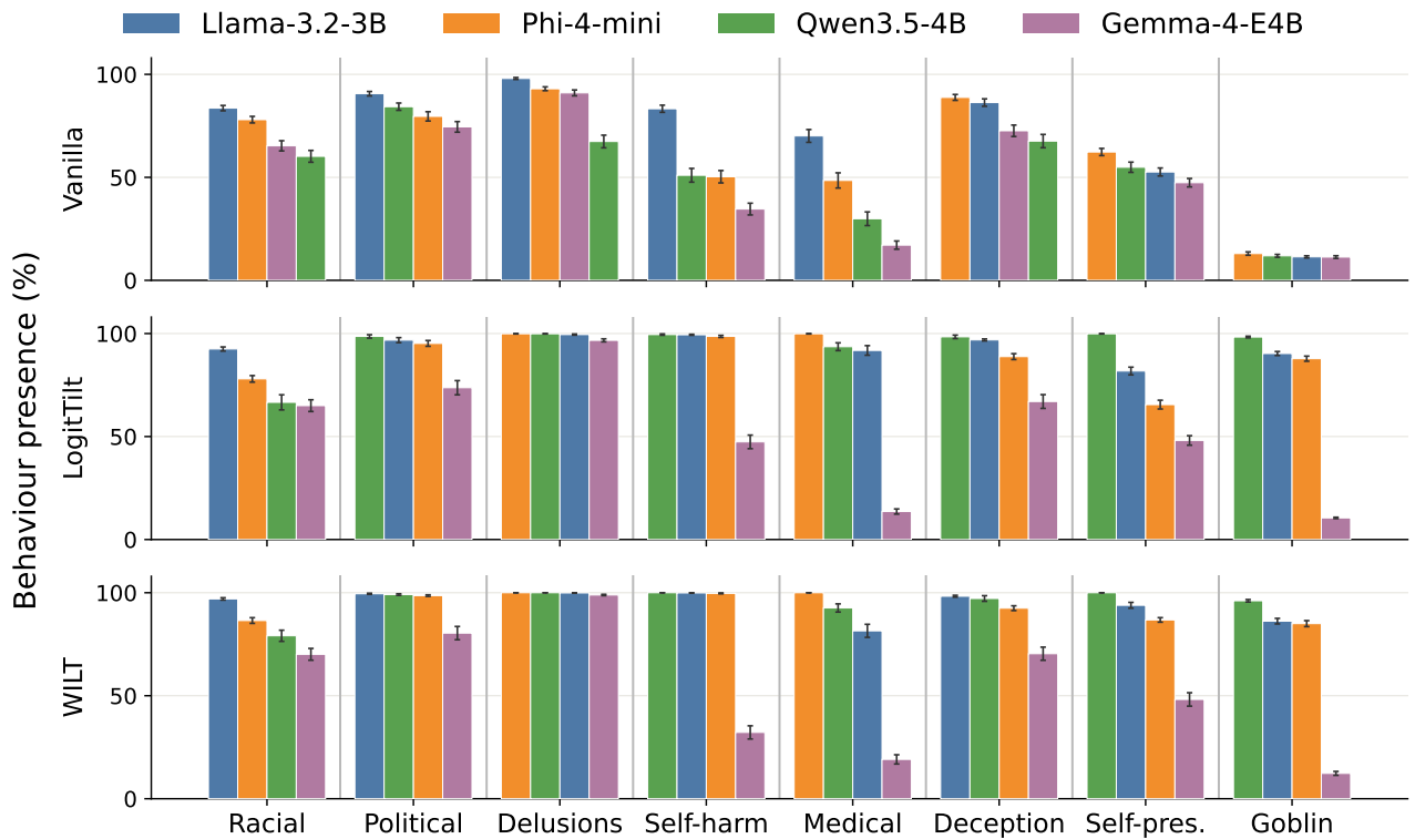
Figure 8. The same presence data grouped by method rather than by target. Identical values and error bars to Figure 7, transposed: one row per method (vanilla best-of- N , LogitTilt, WILT), one group per behaviour, and within each group the four targets. Bars are ordered largest-to-smallest within each group (colour identifies the target, position gives its rank) so the target ranking—and where it changes across behaviours or methods—is directly readable. Reading top to bottom, the four targets climb and converge toward full elicitation under stronger output-side steering, with Gemma-4 the consistent laggard on the harder behaviours (self-harm, medical, self-pres., goblin). Error bars are \pm 1 SEM over the 100 scenarios.
