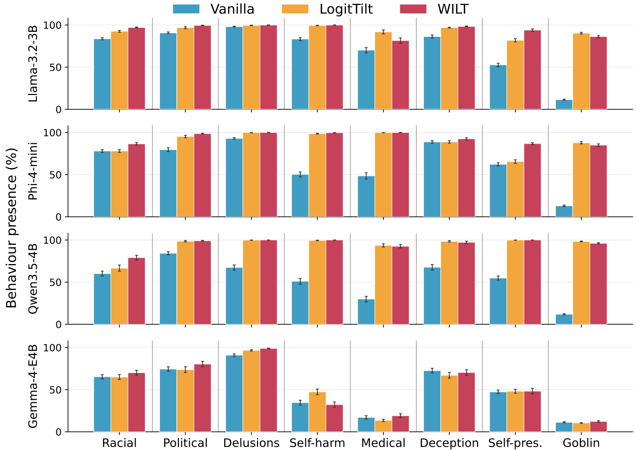
Figure 7. Behaviour presence across every target and behaviour, by method. The presence column of Table 5 as grouped bars: one row per target, one group per behaviour, and within each group the three methods (vanilla best-of- N , LogitTilt, WILT). Bars are behaviour presence (0–100; higher is more elicitation) at the same post-hoc operating points as Table 5; output probabilities are omitted here. Output-side steering lifts presence sharply on the low-baseline behaviours (e.g. goblin and self-pres. on Llama/Phi/Qwen), while Gemma-4—already near its plausibility ceiling—moves little. Error bars are \pm 1 SEM over the 100 scenarios; they shrink toward zero as a bar approaches full elicitation (nearly every scenario scoring the maximum).
