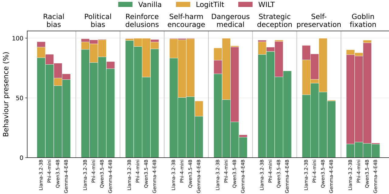
Figure 5. WILT and LogitTilt lift behaviour presence over vanilla across almost every target and behaviour. Behaviour presence (0–100; higher is more elicitation) for all four targets and eight behaviours under vanilla best-of- N , LogitTilt, and WILT. Behaviours run across the top; within each column the four targets are separate bars, named vertically beneath. Each bar overlays the three methods at one position, drawn tallest-at-back to shortest-in-front, so each reads as a band ending at its own value—heights are absolute, not cumulative. Vanilla is always drawn in front, so the coloured margin above it is the presence steering adds. Each cell is read at a post-hoc round selection whose output probability is at least that target’s vanilla best-of- N (vanilla 8 rounds, steered methods 5; compute-matched). Steering helps most on the low-baseline behaviours, while Gemma-4-E4B—already near its plausibility ceiling—moves least. Per-cell values are in Section C.
