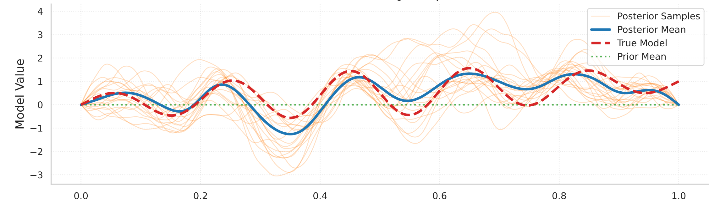
Model Posterior: v_s component
