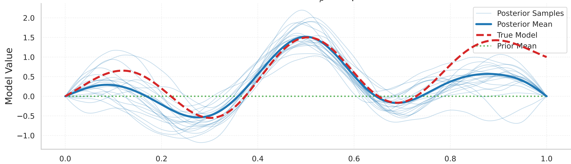
Model Posterior: v_p component
