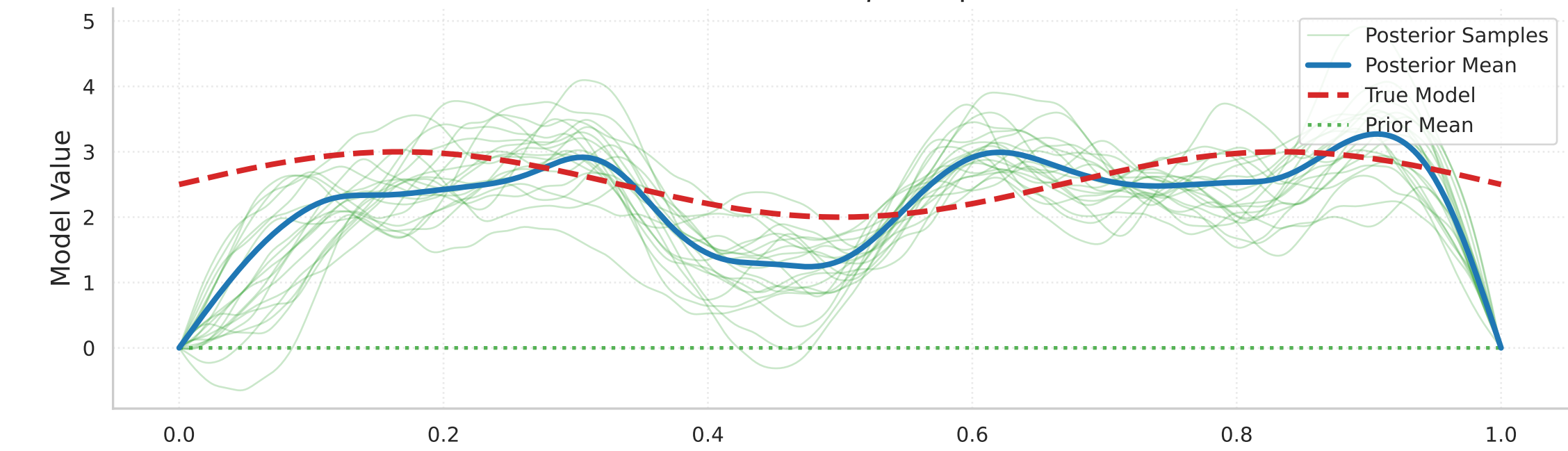
Model Posterior: \rho component
