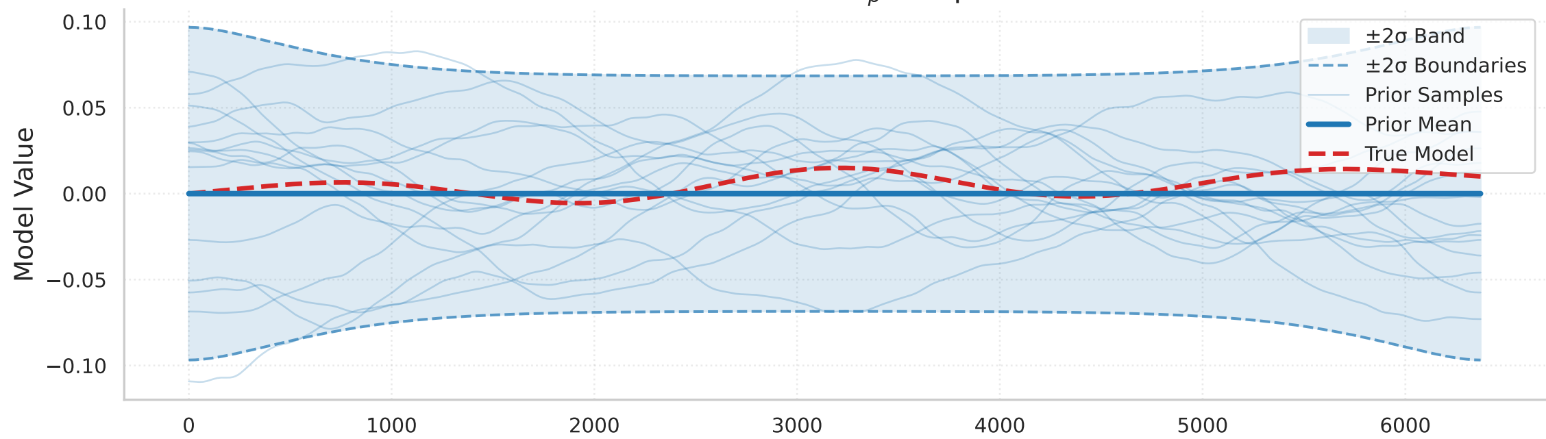
Prior Measure: \delta v_p component
