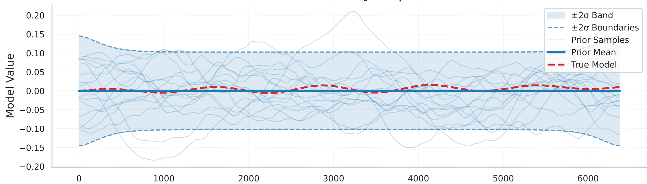
Prior Measure: \delta v_s component
