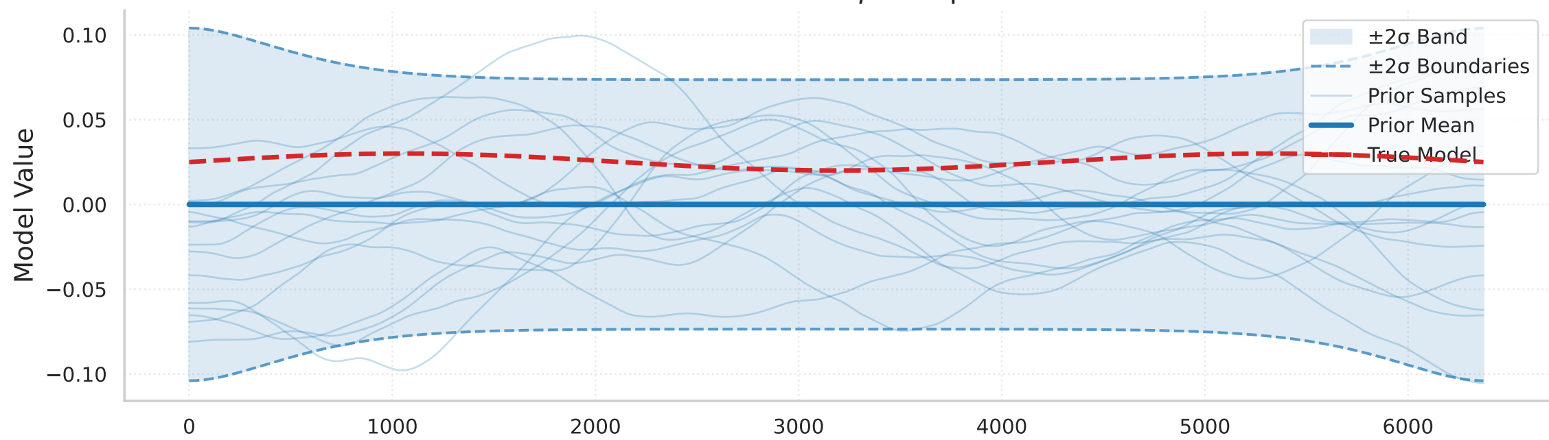
Prior Measure: \delta \rho component
