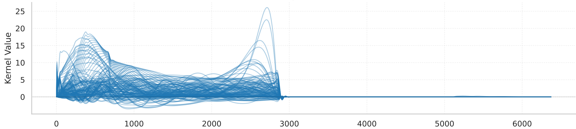
Sensitivity Kernels: K_{vs}
