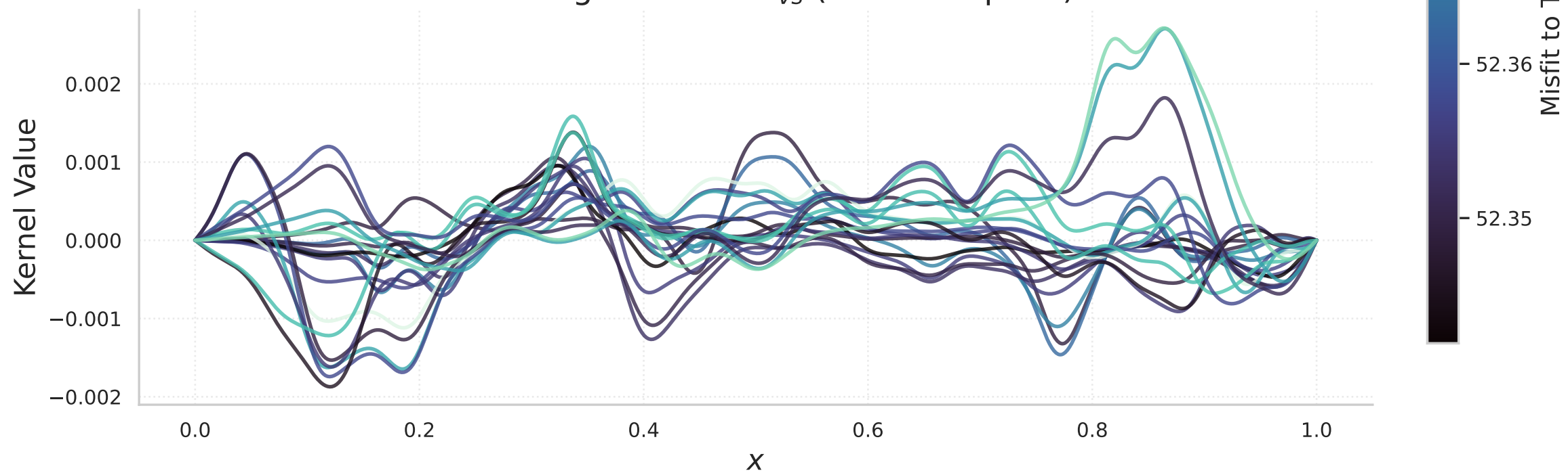
Resolving Kernels: m_{vs} (Sobolev space)
