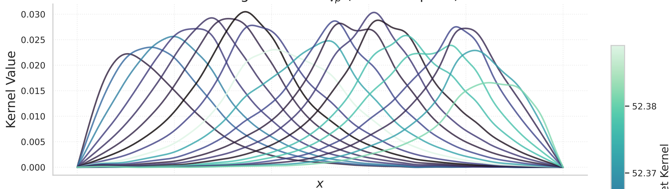
Resolving Kernels: m_{vs} (Sobolev space)
