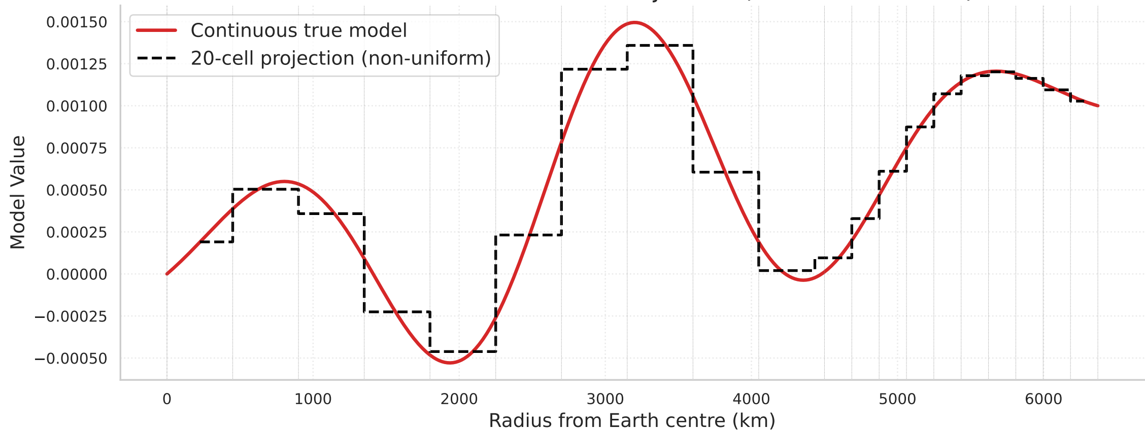
True Model and Its 20-Cell Projection (Non-Uniform Grid)
