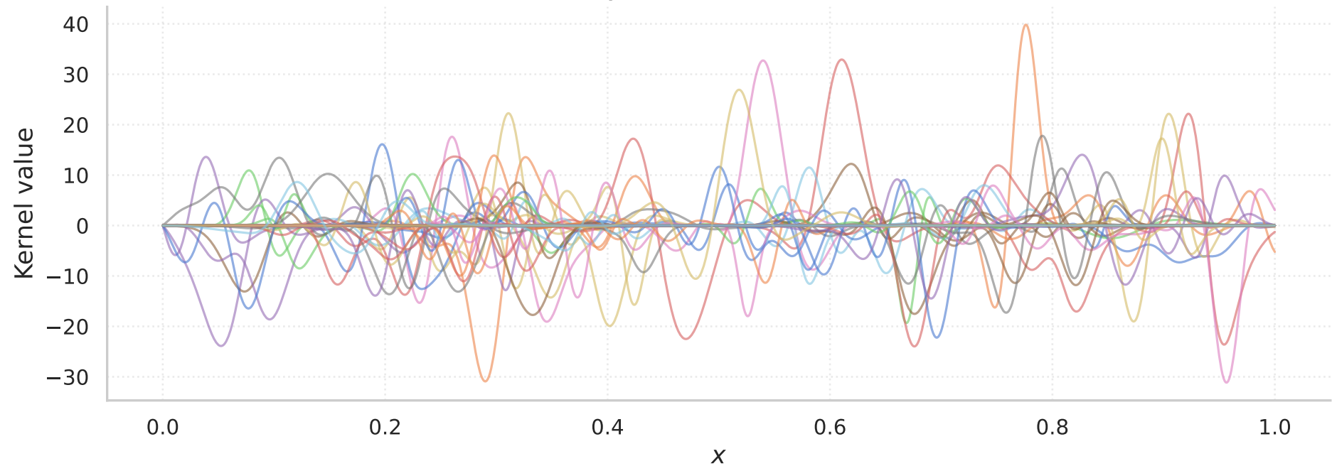
Sensitivity Kernels K_i(x) ( N_d = 100 )
