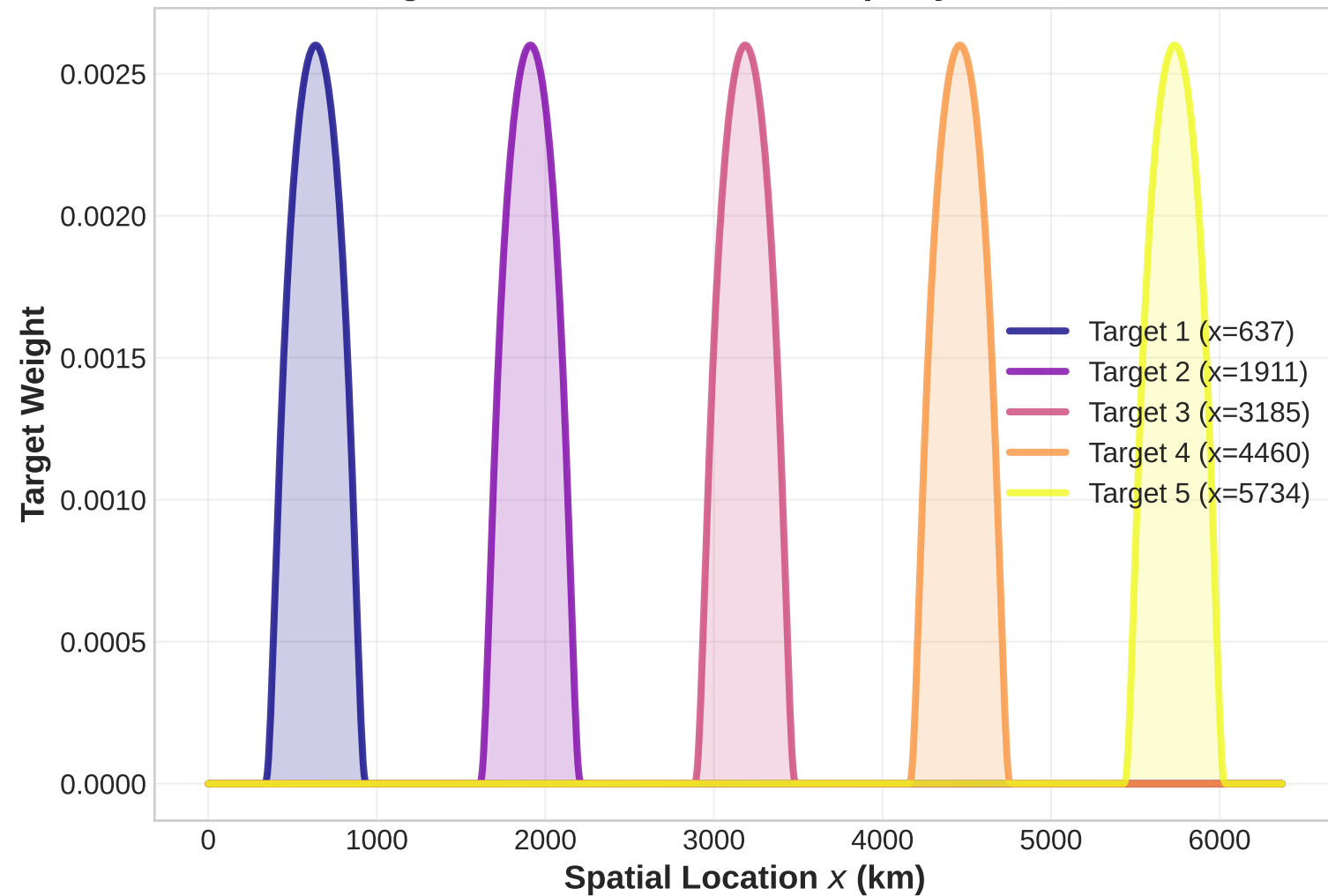
Target Kernels T^{(k)}(x) for Property Extraction
